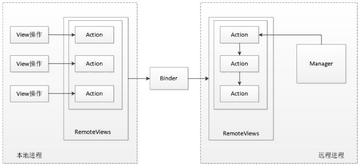
图5-3 RemoteViews跨进程交互
