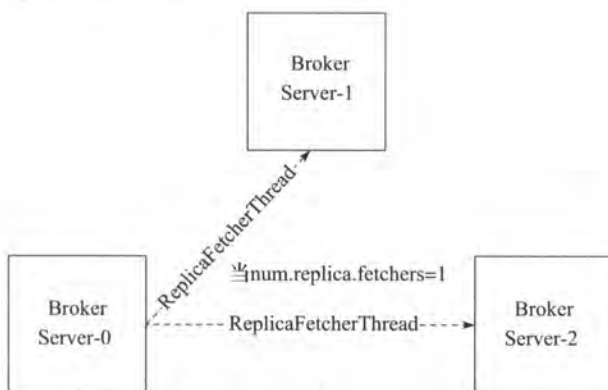
图 4-11 ReplicaFetcherThread
