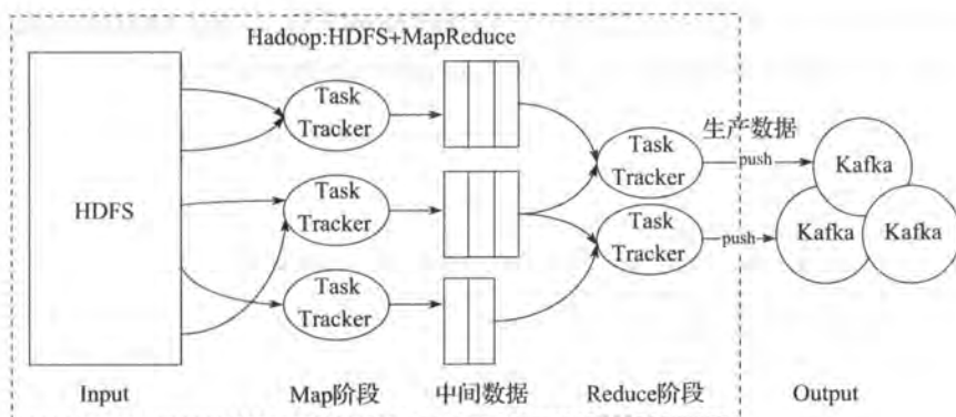
图 9-11 Hadoop-Producer
