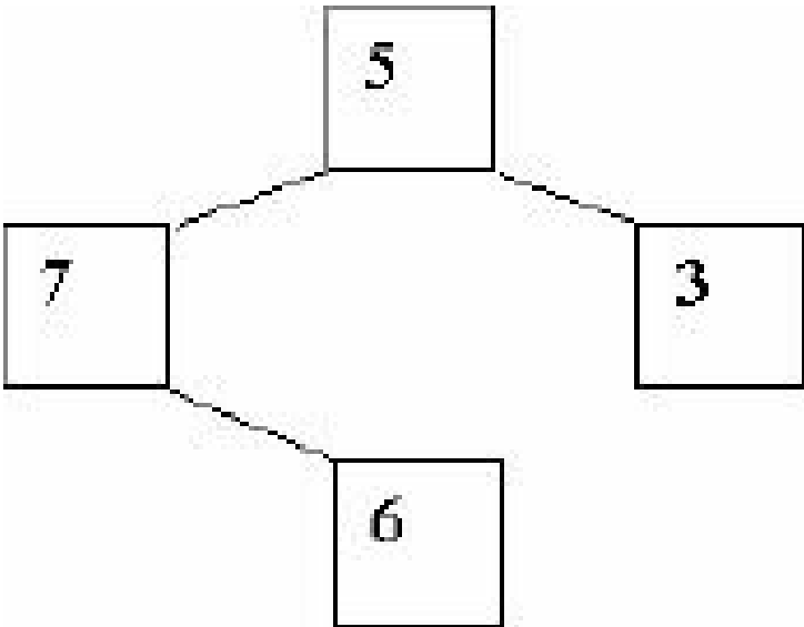
图6-7 结点权值
