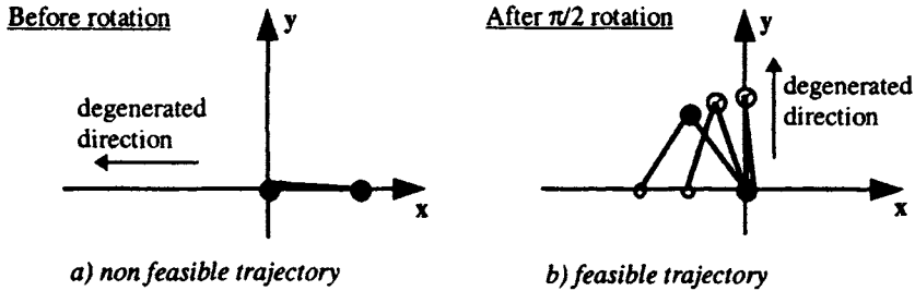
Figure 6.2. Motion in the null space of J
