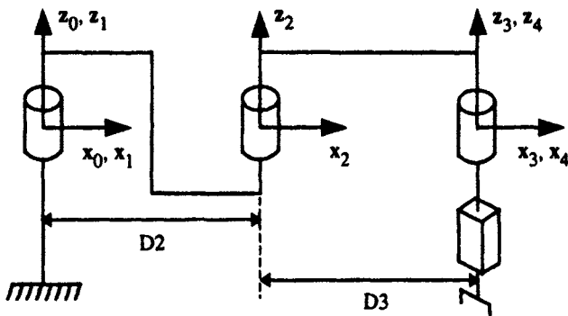
Figure 3.4. SCARA Robot
