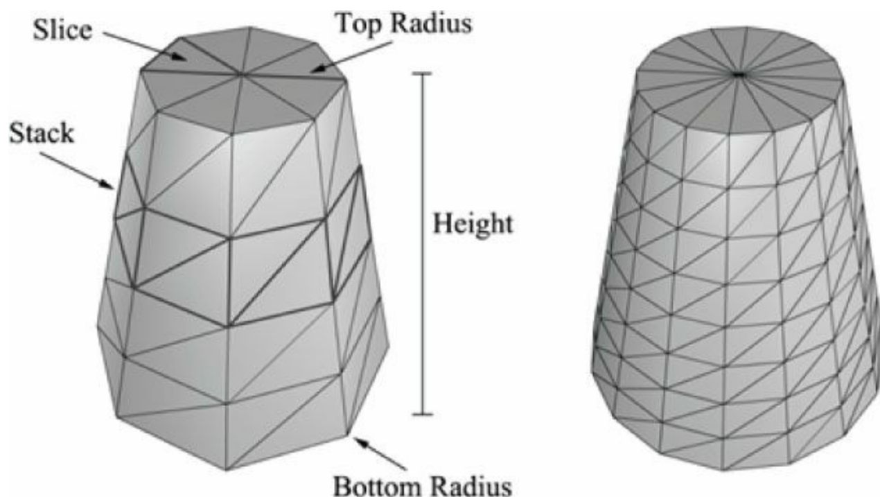
Figure 6.13. In this illustration, the cylinder on the left has 8 slices and 4 stacks, and the cylinder on the right has 16 slices and 8 stacks. The slices and stacks control the triangle density. Note that the top and bottom radii can differ so that we can create cone shaped objects, not just “pure” cylinders.
