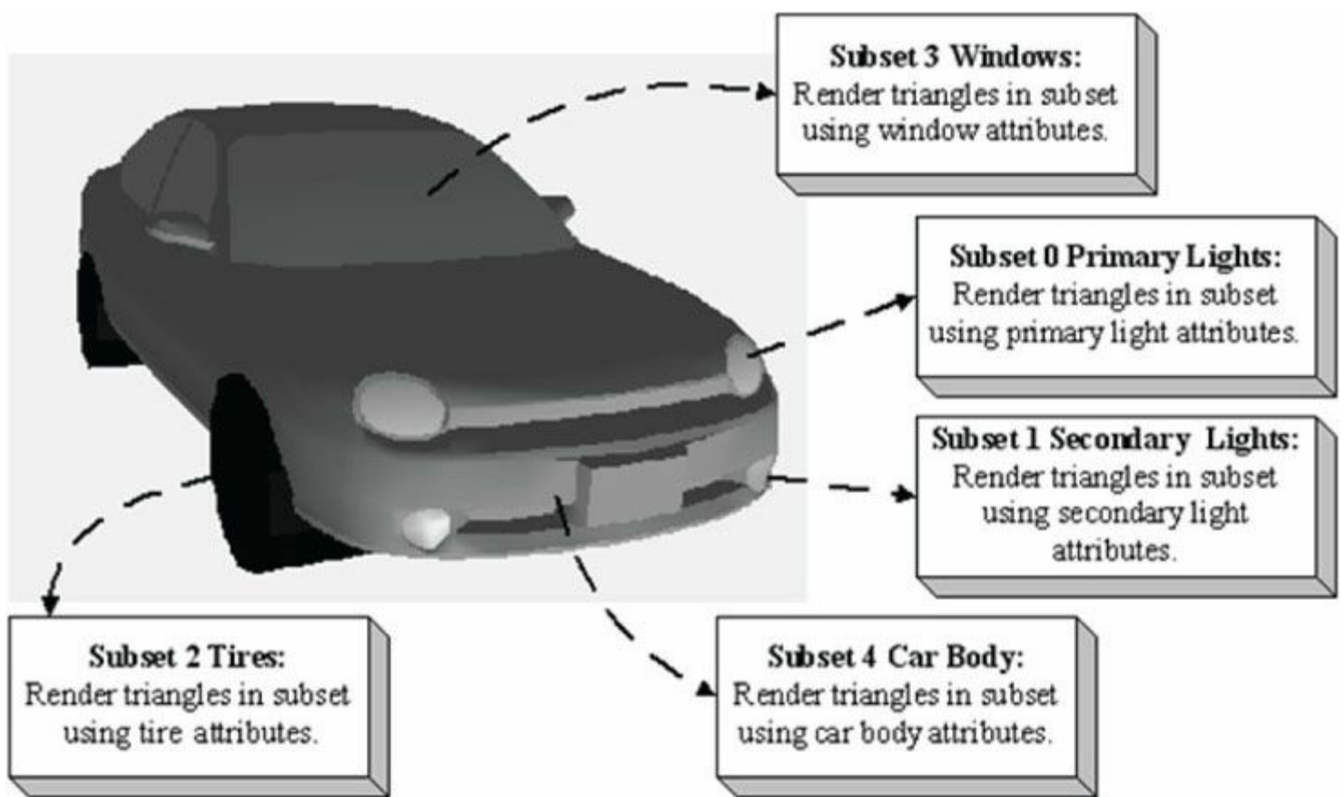
Figure 7.16. A car mesh divided into five material attribute groups.
