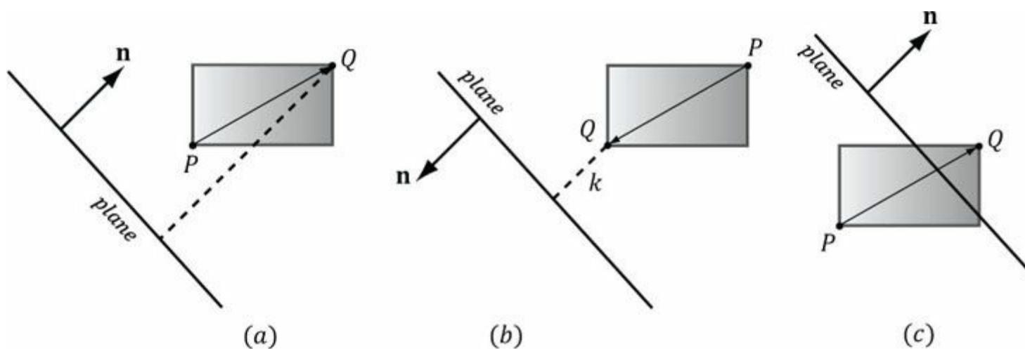
Figure 15.8. ABB/plane intersection test. The diagonal \overrightarrow{PQ} is always the diagonal most directed with the plane normal.
