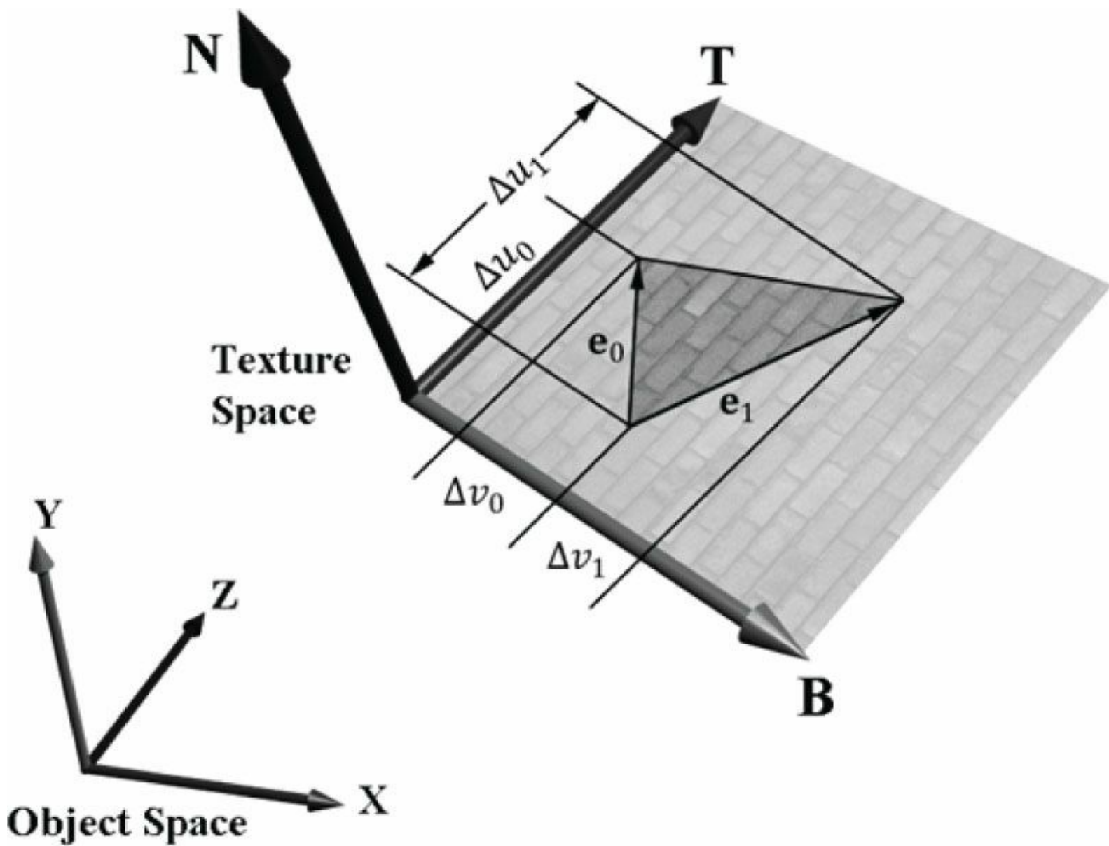
Figure 18.4. The relationship between the texture space of a triangle and the object space. The 3D tangent vector T aims in the u -axis direction of the texturing coordinate system, and the 3D tangent vector B aims in the v -axis direction of the texturing coordinate system.
