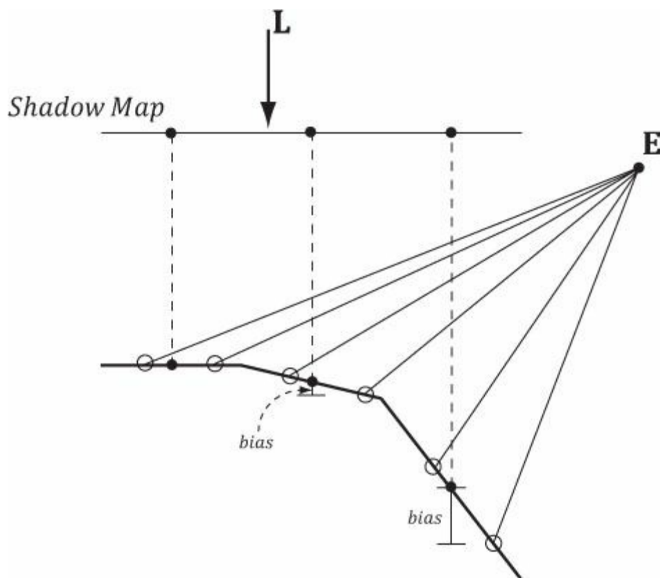
Figure 21.11. Polygons with large slopes, relative to the light source, require more bias than polygons with small slopes relative to the light source.
