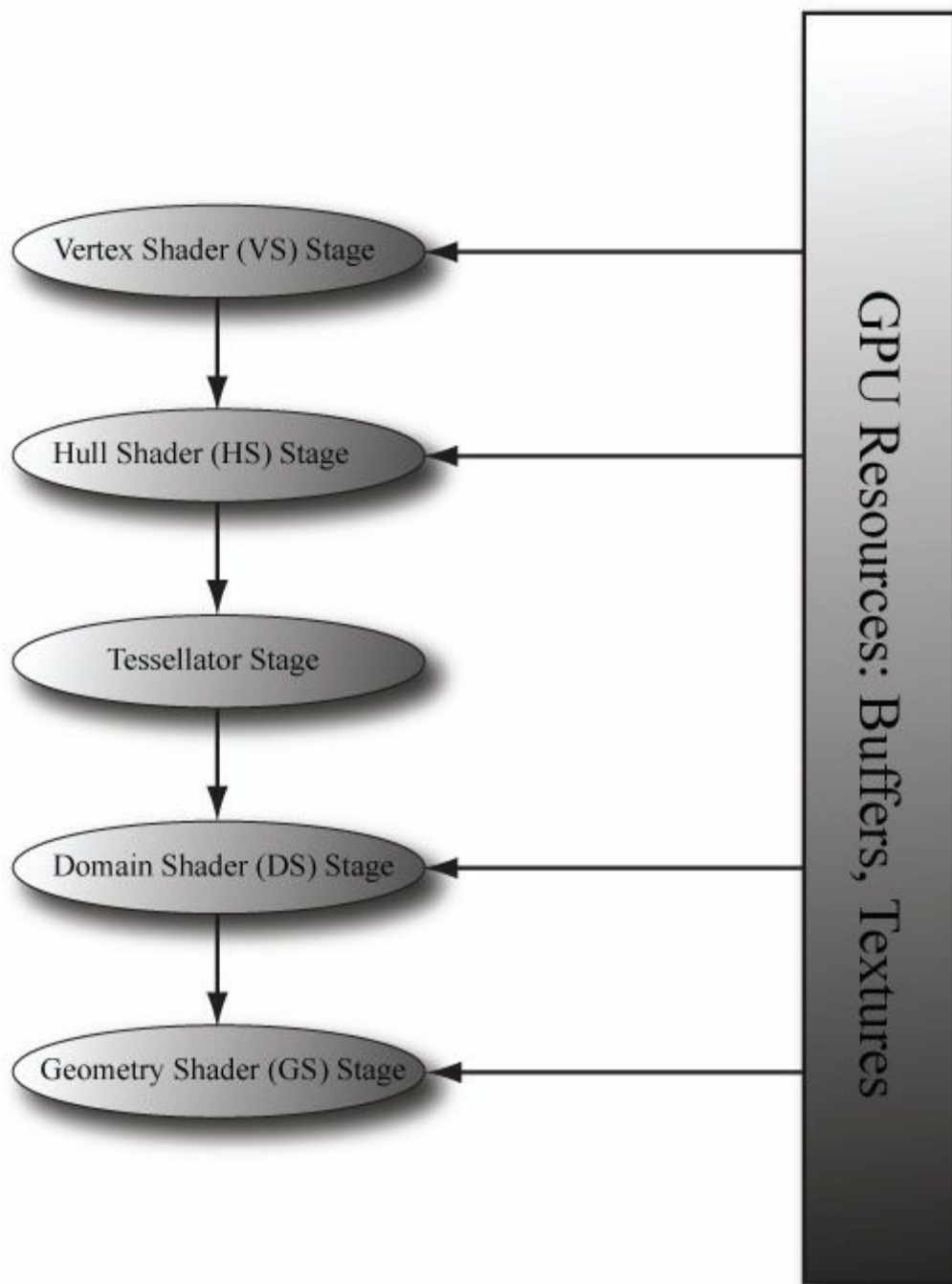
Figure 13.1. A subset of the rendering pipeline showing the tessellation stages.
