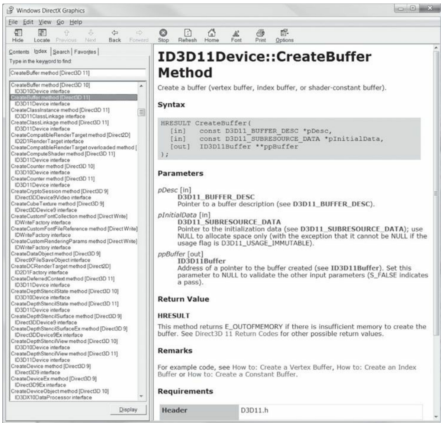
Figure 2. Index of the DirectX documentation.
