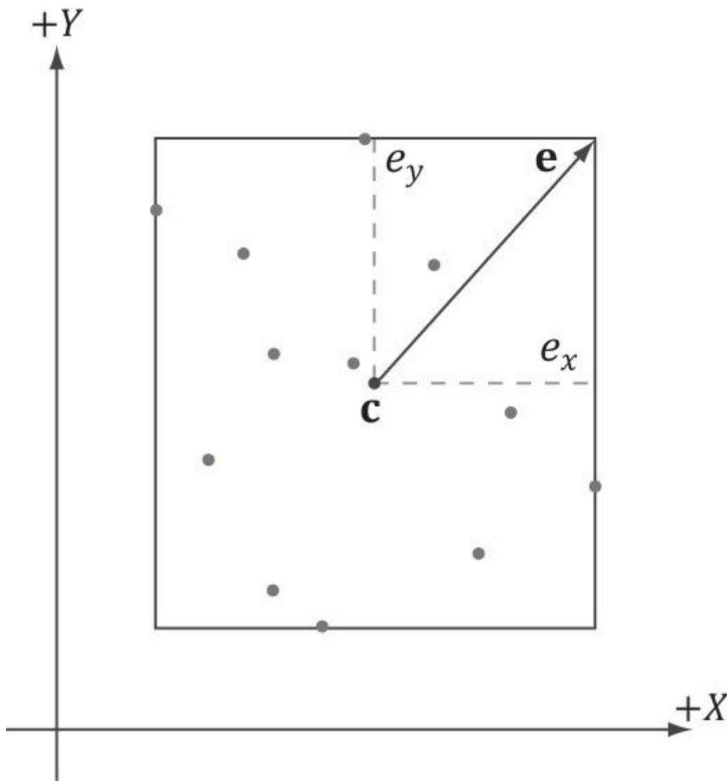
Figure 15.3. The AABB of a set of points using center and extents representation.
