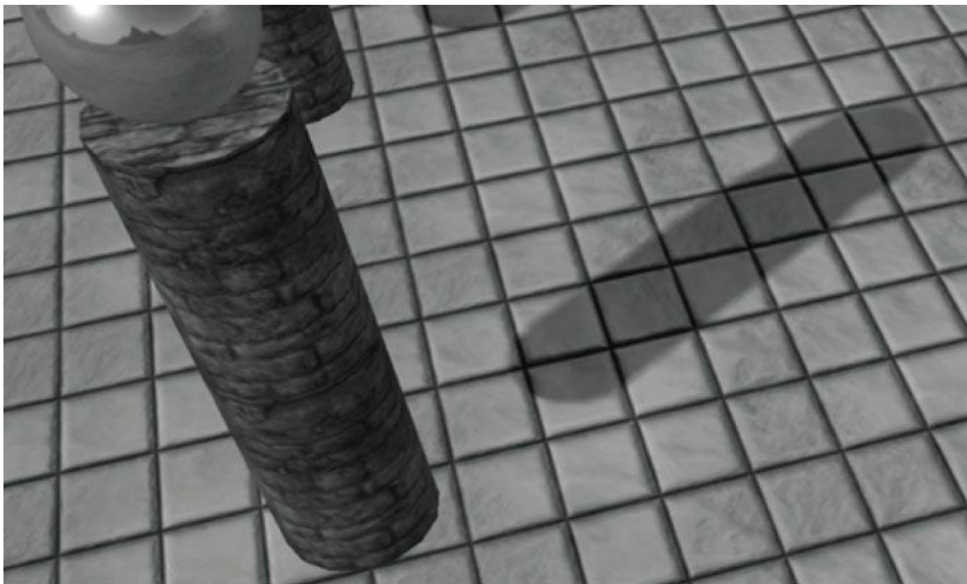
Figure 21.10. Peter-panning—the shadow becomes detached from the column due to a large depth bias.
