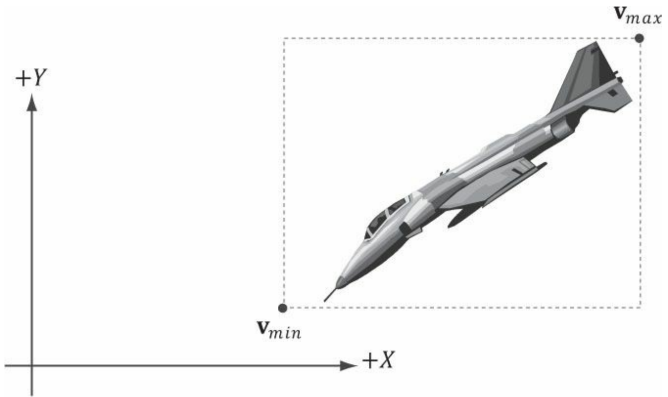
Figure 15.5. The bounding box is axis aligned with the XY -frame.
