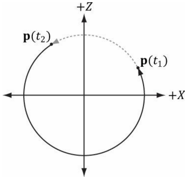
Figure 4.9. If we paused at t_1 and unpaused at t_2 , and counted paused time, then when we unpause, the position will jump abruptly from p(t_1) to p(t_2) .
