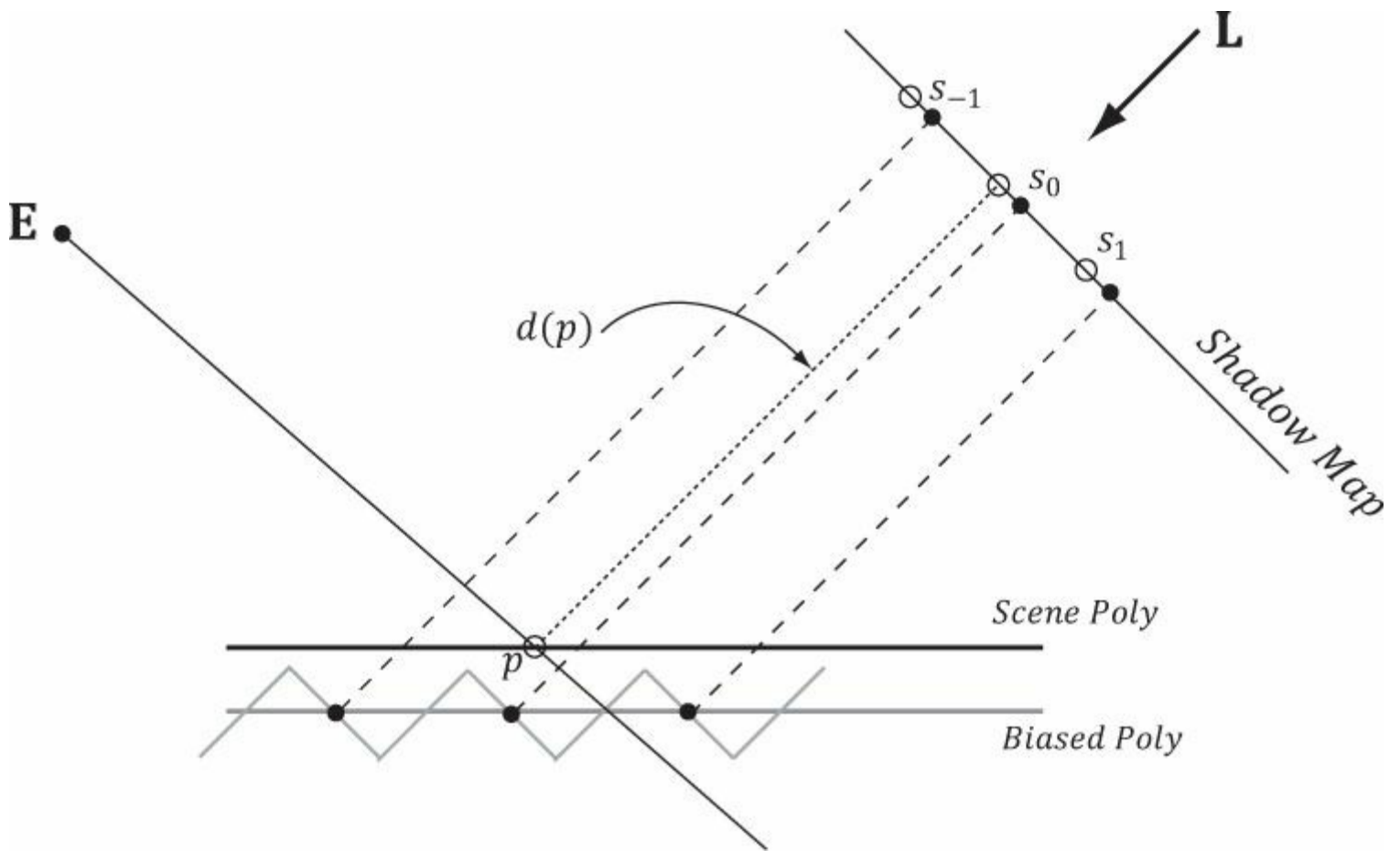
Figure 21.16. Comparing the depth d(p) with s_0 is correct, because the texel s_0 covers the scene area p is contained in. However, it is not correct to compare d(p) with s_{-1} and s_1 , as those texels cover areas of the scene that are unrelated to p .
