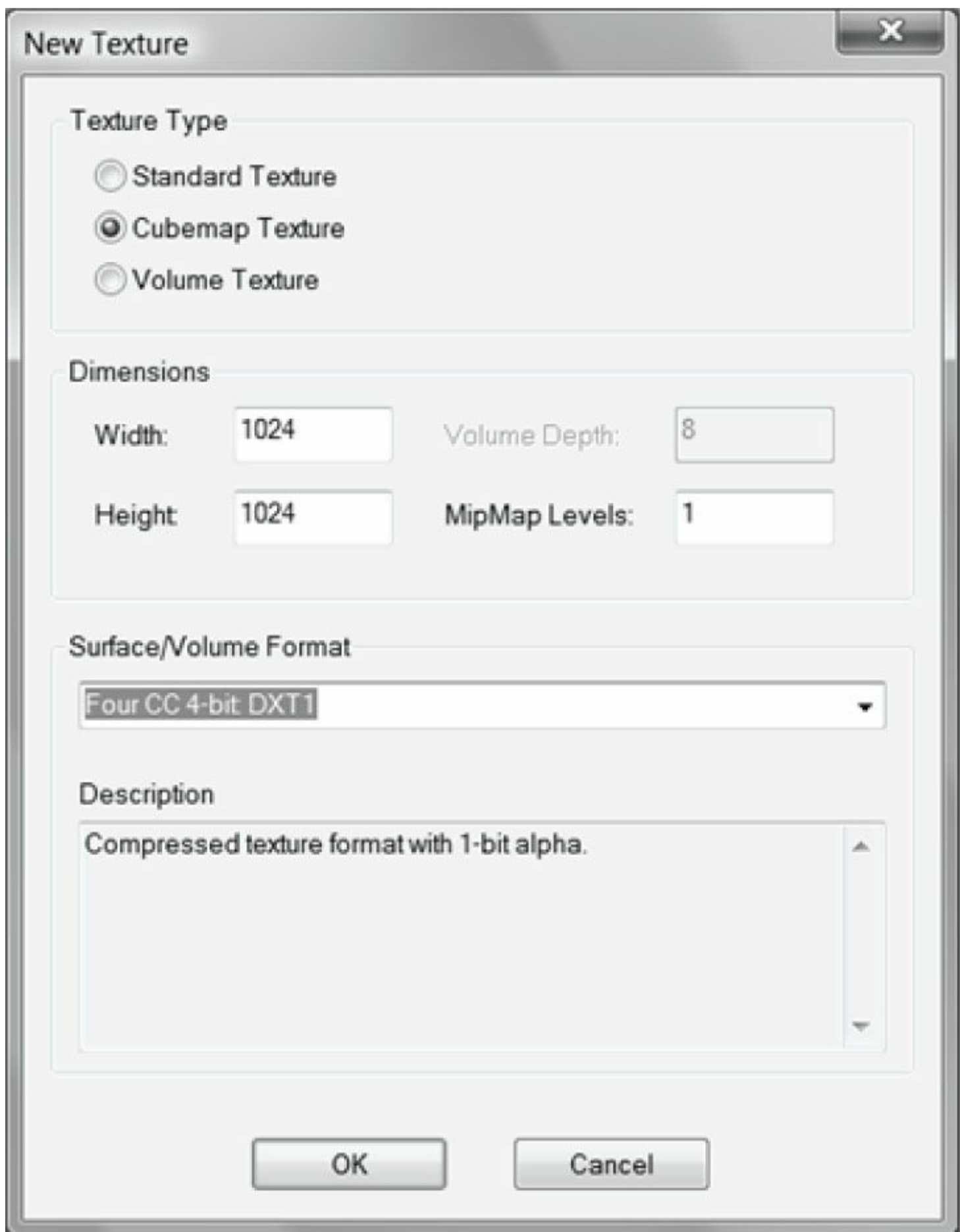
Figure 17.4. Creating a new cube texture with the DirectX Texture Tool.
