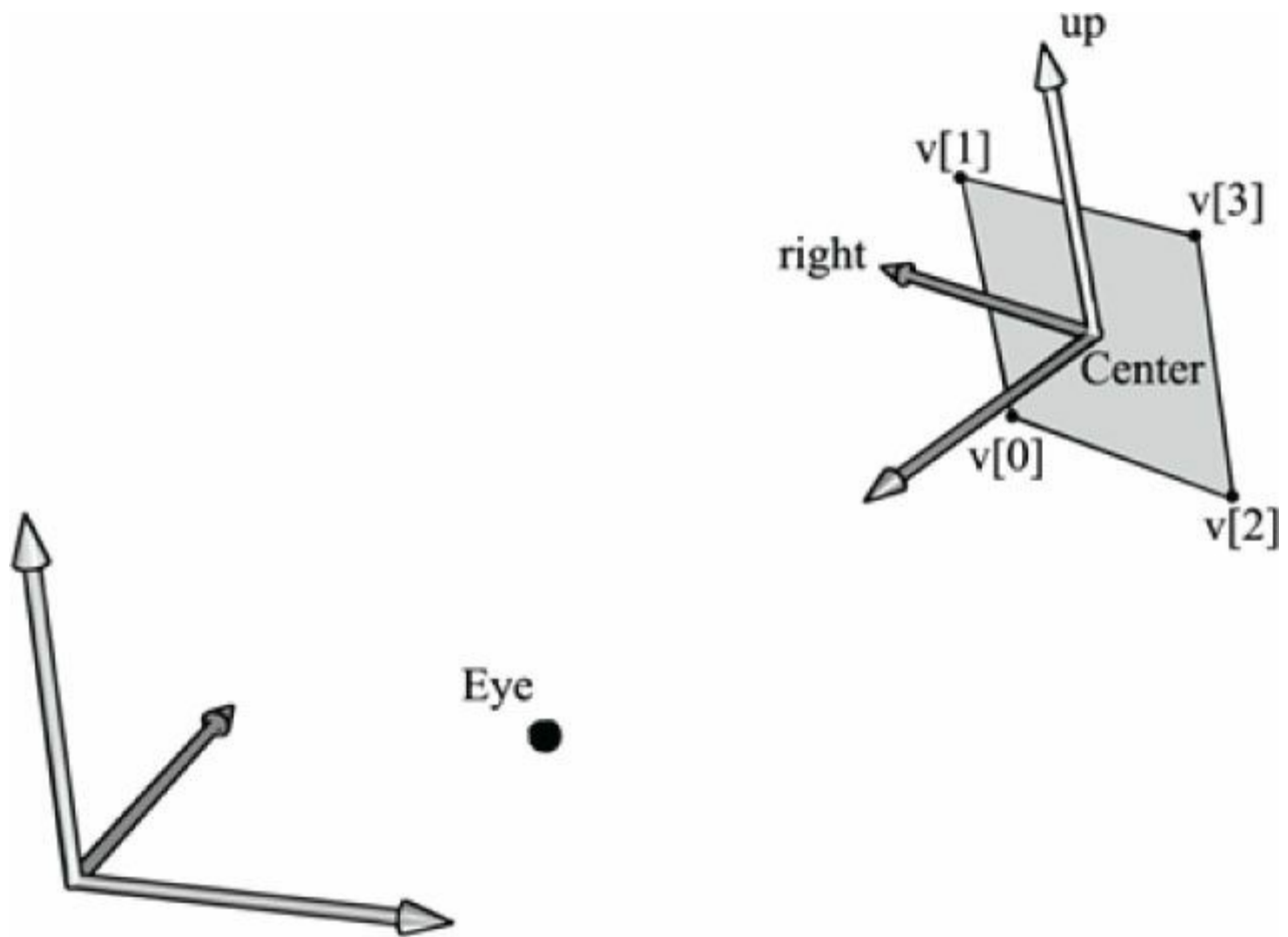
Figure 11.4. Computing the billboard quad vertices from the local coordinate system and world size of the billboard.
