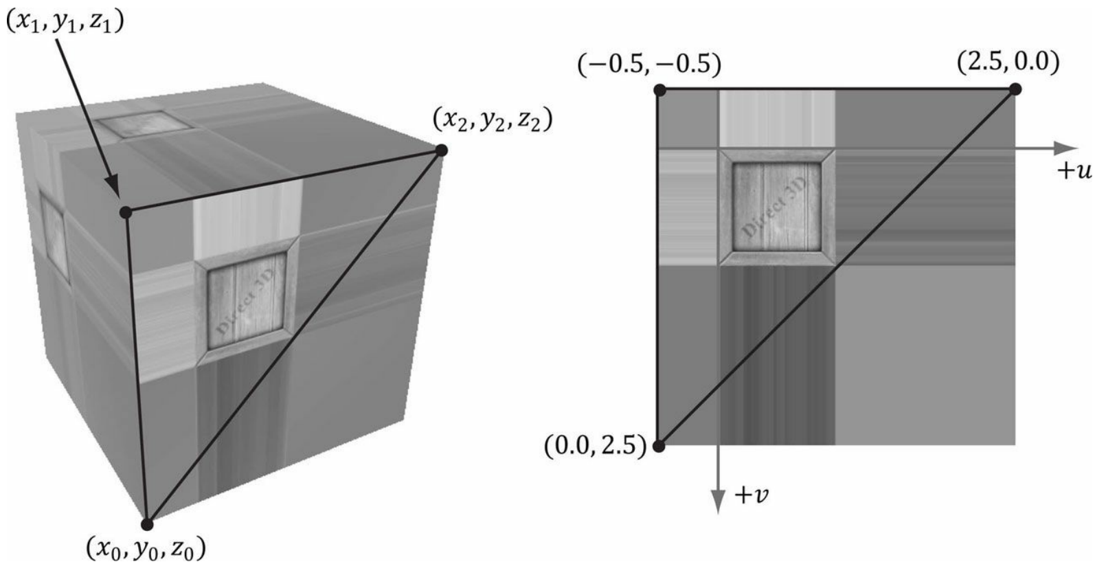
Figure 8.12. Clamp address mode.
