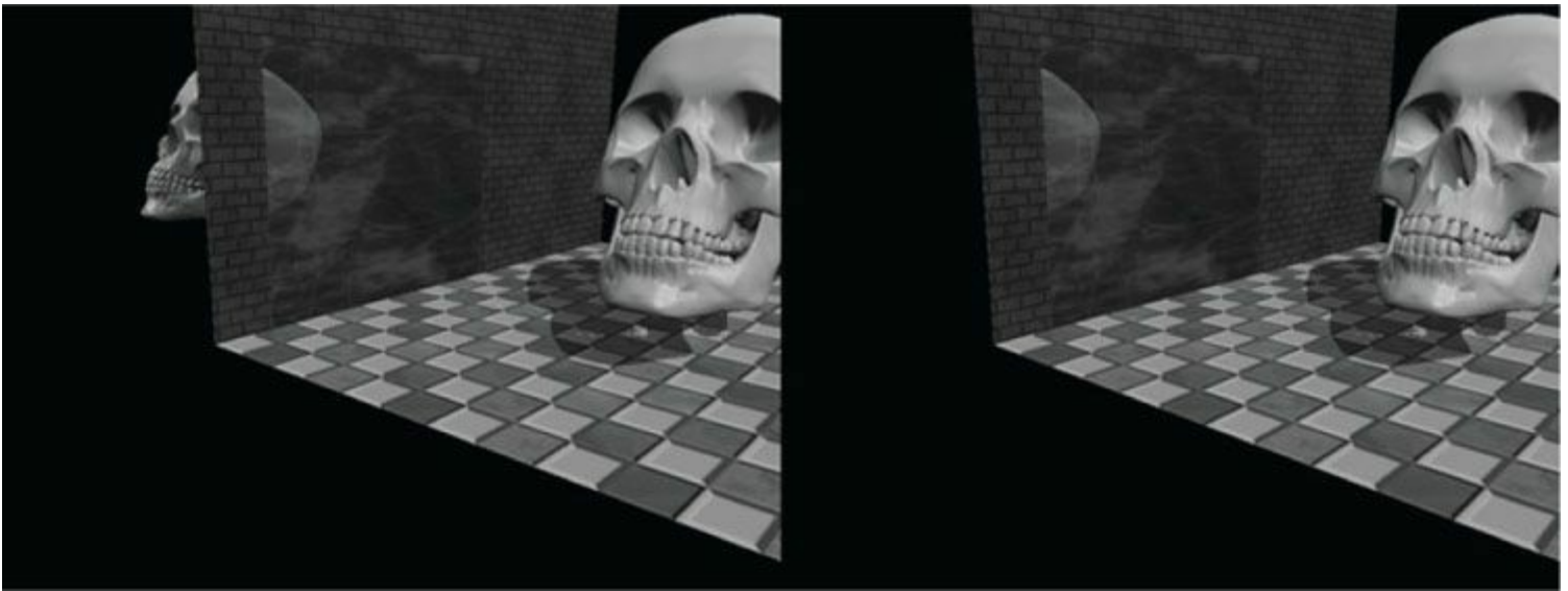
Figure 10.1. (Left) The reflected skull shows properly in the mirror. The reflection does not show through the wall bricks because it fails the depth test in this area. However, looking behind the wall we are able to see the reflection, thus breaking the illusion (the reflection should only show up through the mirror). (Right) By using the stencil buffer, we can block the reflected skull from being rendered unless it is being drawn in the mirror.
