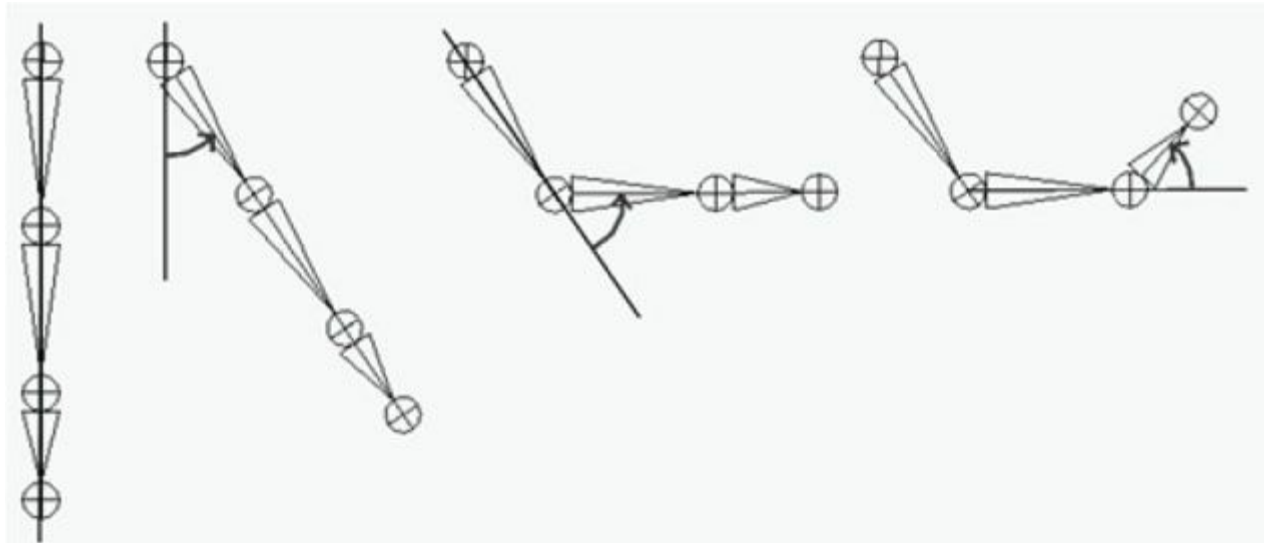
Figure 25.1. Hierarchy transforms; observe that the parent transformation of a bone influences itself and all of its children.
