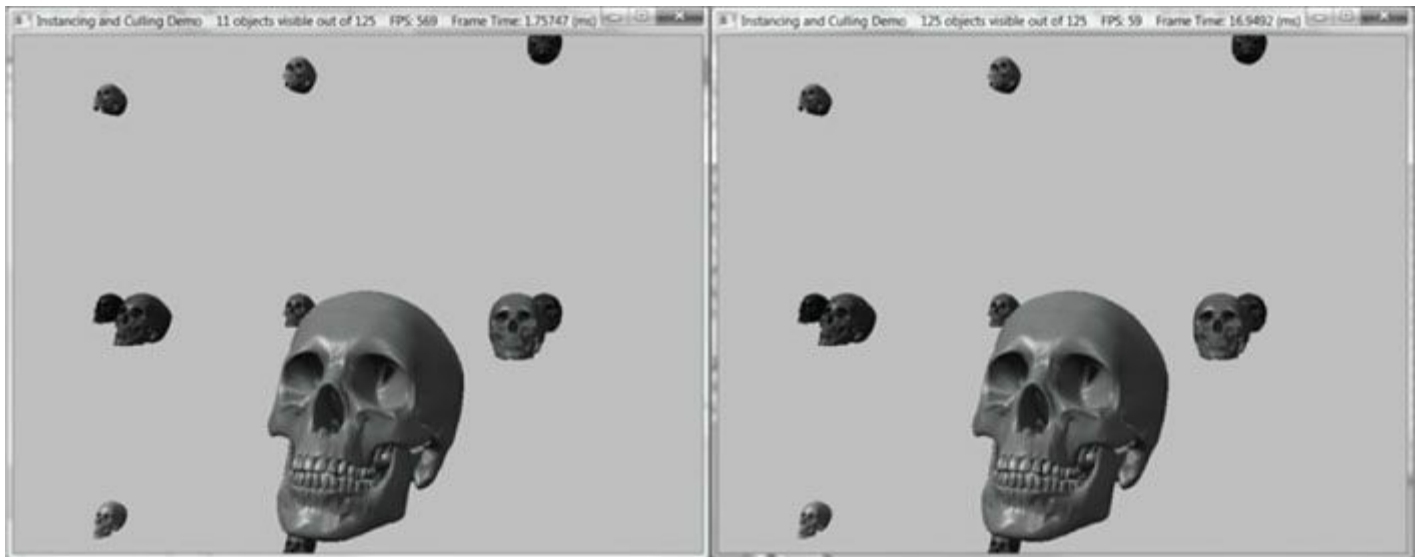
Figure 15.12. (Left) Frustum culling is turned on, and we see that 11 out of 125 instances are visible, and it takes about 1.75 ms to render a frame. (Right) Frustum culling is turned off, and we are rendering all 125 instances, and it takes about 16.94 ms to render a frame—9.68 times longer than when frustum culling is enabled.
