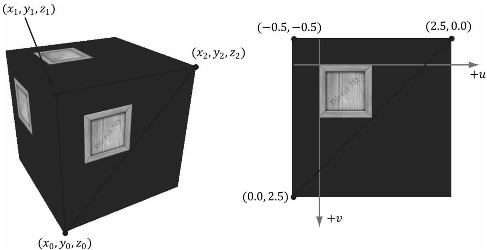
Figure 8.11. Border color address mode.
