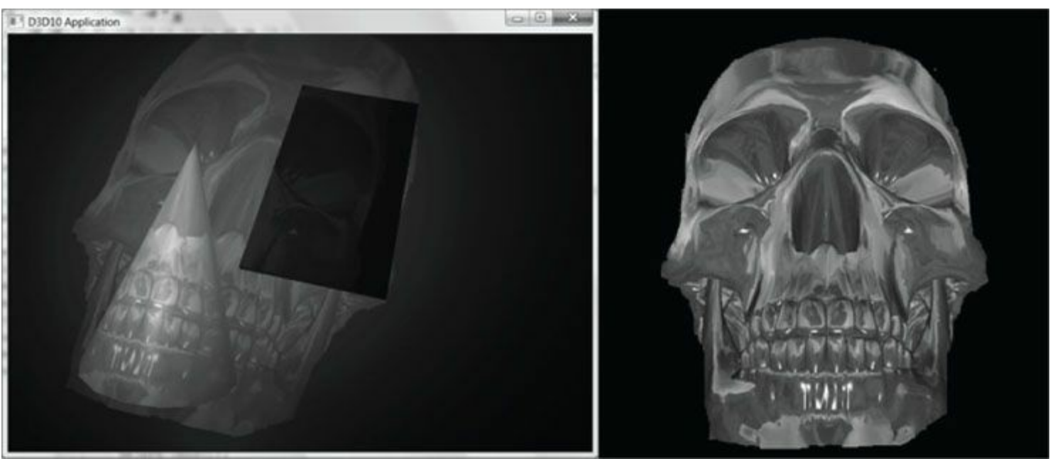
Figure 21.3. The skull texture (right) is projected onto the scene geometry (left).
