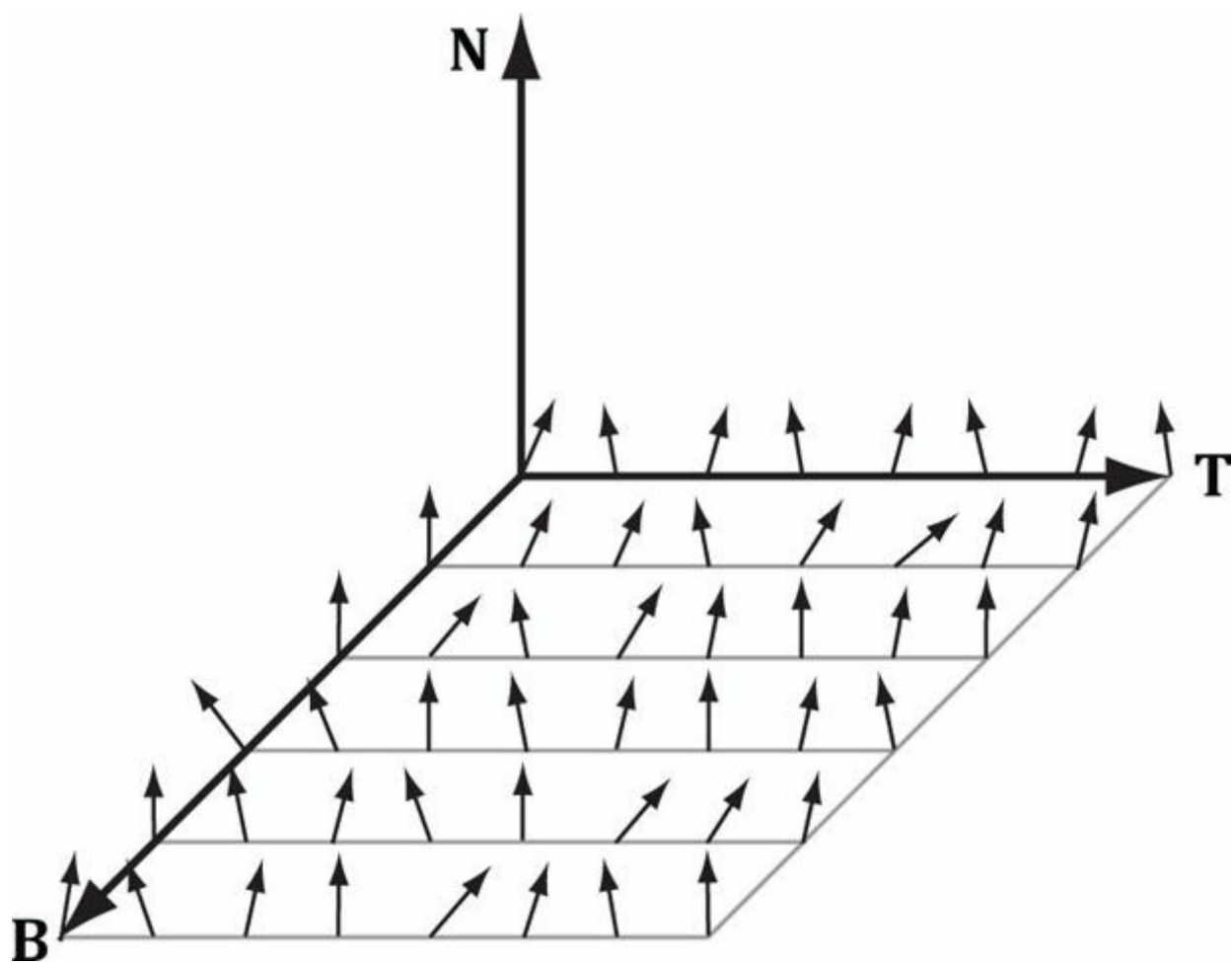
Figure 18.3. Normals stored in a normal map relative to a texture space coordinate system defined by the vectors T (x-axis), B (y-axis), and N (z-axis). The T vector runs right horizontally to the texture image; the B vector runs down vertically to the texture image; and N is orthogonal to the texture plane.
