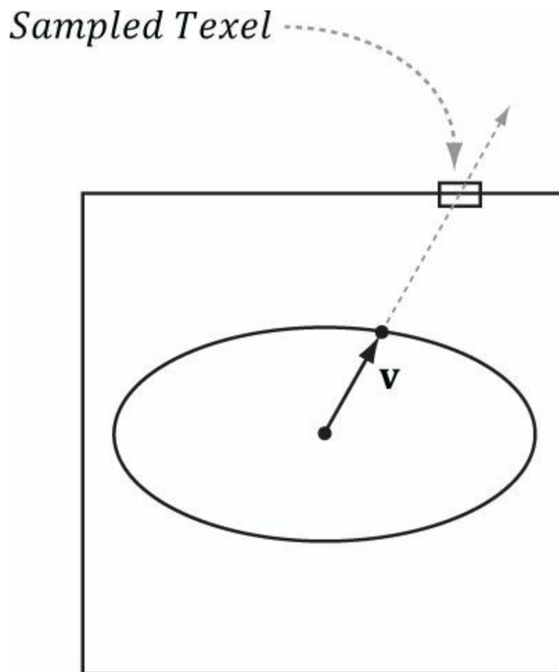
Figure 17.6. We illustrate in 2D for simplicity; in 3D the square becomes a cube and the ellipse becomes an ellipsoid. We assume that the sky and environment map are centered about the same origin. Then to texture a point on the surface of the ellipsoid, we use the vector from the origin to the surface point as the lookup vector into the cube map. This projects the cube map onto the ellipsoid.
