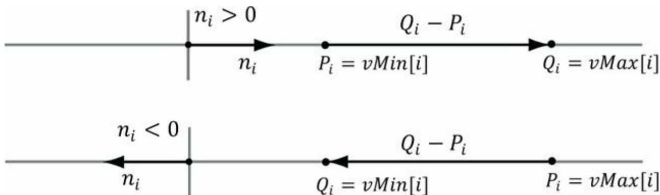
Figure 15.9. (Top) The normal component along the i th axis is positive, so we choose P_i = vMin[i] and Q_i = vMax[i] so that Q_i - P_i has the same sign as the plane normal coordinate n_i . (Bottom) The normal component along the i th axis is negative, so we choose P_i = vMax[i] and Q_i = vMin[i] so that Q_i - P_i has the same sign as the plane normal coordinate n_i .
