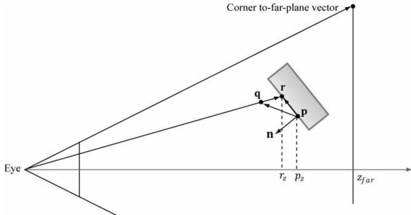
Figure 22.6. If \mathbf{r} lies on the same plane as \mathbf{p} , it can pass the first condition that the distance |p_z - r_z| is small enough that \mathbf{r} occludes \mathbf{p} . However, the figure shows this is incorrect as \mathbf{r} does not occlude \mathbf{p} because they lie on the same plane. Scaling the occlusion by \max\left(\mathbf{n} \cdot \left(\frac{\mathbf{r} - \mathbf{p}}{\|\mathbf{r} - \mathbf{p}\|}\right), 0\right) prevents this
