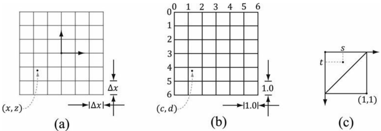
Figure 19.12. (a) The point in the xz -plane relative to the terrain coordinate system has coordinates (x, z) . (b) We pick a new coordinate system where the origin is the upper-left most grid vertex, the positive z -axis goes down, and each unit is scaled so that it corresponds to one cell space. The point has coordinates (c, d) relative to this coordinate system. This transformation involves a translation and scaling. Once in this new coordinate system, finding the row and column of the cell we are in is trivial. (c) We introduce a third coordinate system, which has its origin at the upper-left vertex of the cell the point is in. The point has coordinates (s, t) relative to this coordinate system. Transforming the coordinates into this system involves only a simple translation to offset the coordinates. Observe that if s + t \leq 1 we are in the “upper” triangle, otherwise we are in the “lower” triangle.
