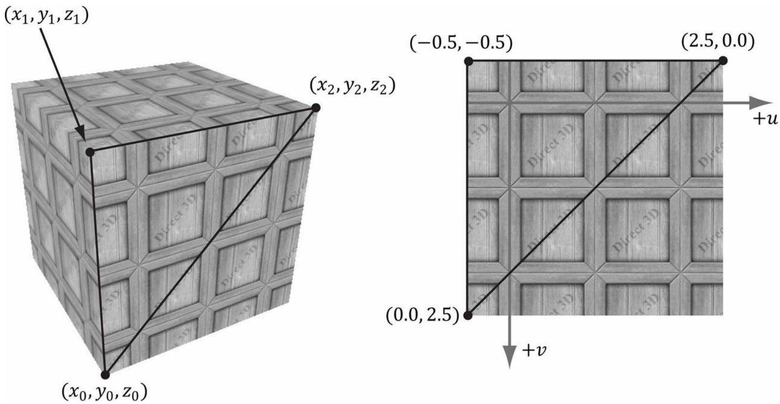
Figure 8.10. Wrap address mode.
