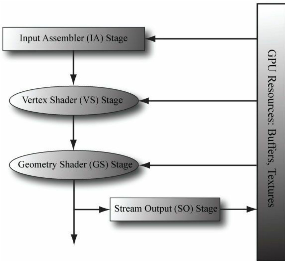
Figure 20.4. Primitives are pumped through the pipeline. The geometry shader outputs primitives which are streamed-out to vertex buffers in GPU memory.
