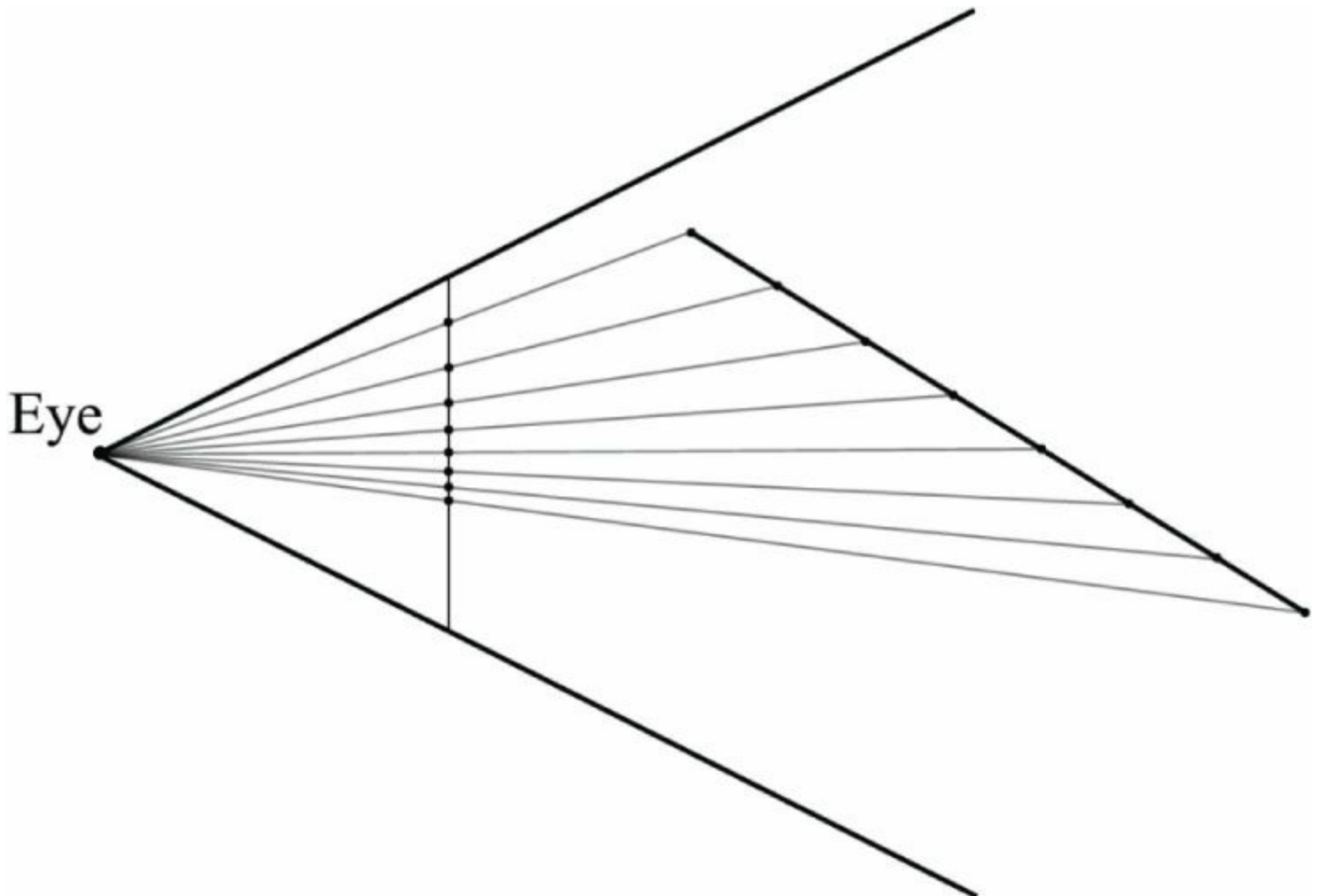
Figure 5.34. A 3D line is being projected onto the projection window (the projection is a 2D line in screen space). We see that taking uniform step sizes along the 3D line corresponds to taking nonuniform step sizes in 2D screen space. Therefore, to do linear interpolation in 3D space, we need to do nonlinear interpolation in screen space.
