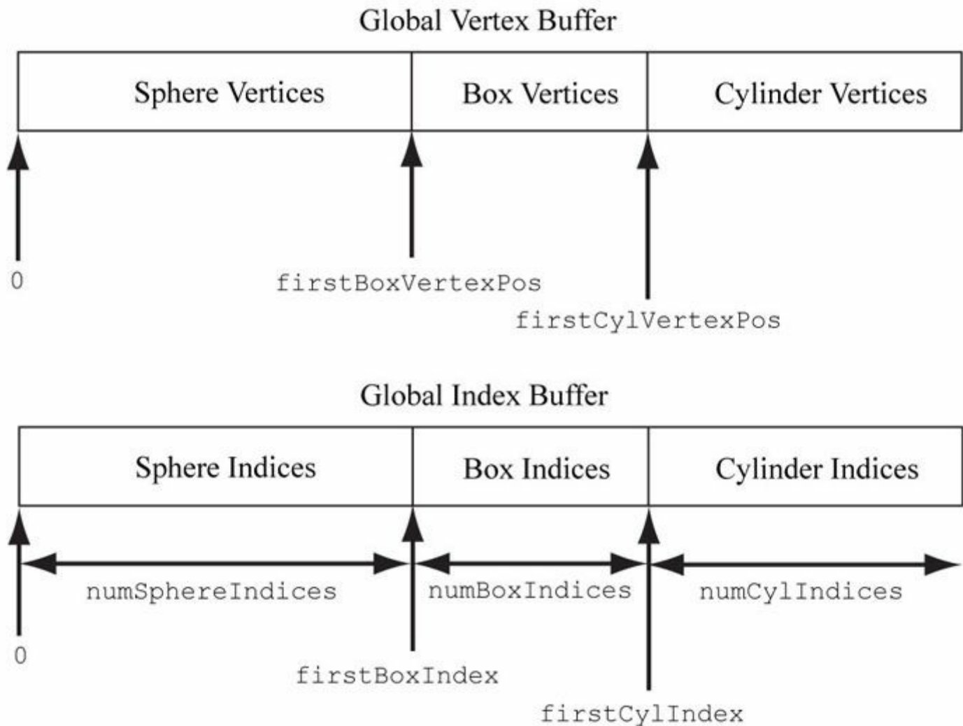
Figure 6.3. Concatenating several vertex buffers into one large vertex buffer, and concatenating several index buffers into one large index buffer.
