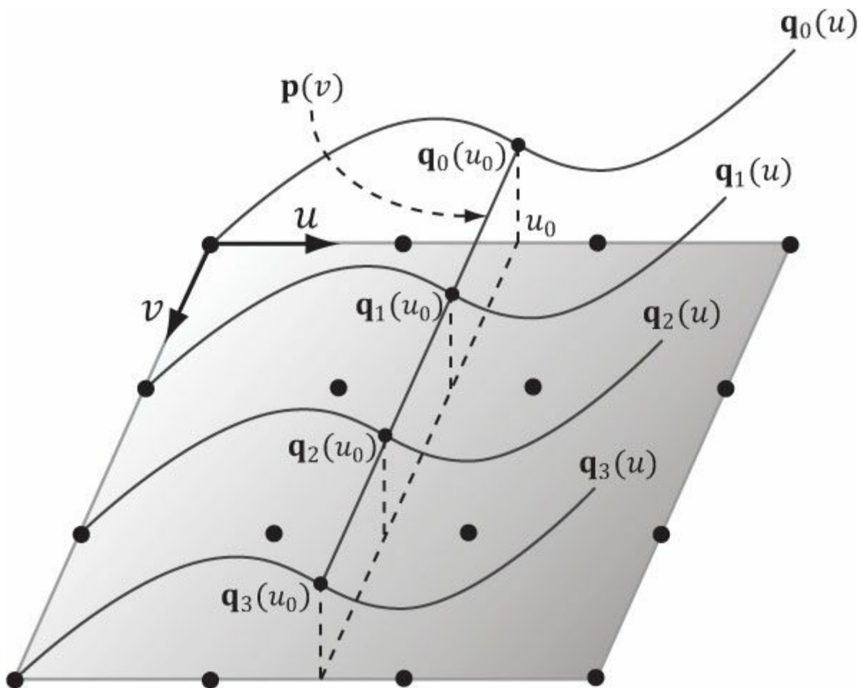
Figure 13.7. Constructing a Bézier surface. Some simplifications were made to make the figure easier to understand—the control points do not all lie in the plane, all the \mathbf{q}_i(u) need not be the same as the figure suggests (they would only be the same if the control points were the same for each row to give the same curves), and \mathbf{p}(v) generally would not be a straight line but a cubic Bézier curve.
