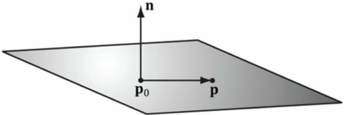
Figure C.6. A plane defined by a normal vector \mathbf{n} and a point \mathbf{p}_0 on the plane. If \mathbf{p}_0 is a point on the plane, then the point \mathbf{p} is also on the plane if and only if the vector \mathbf{p} - \mathbf{p}_0 is orthogonal to the plane's normal vector.
