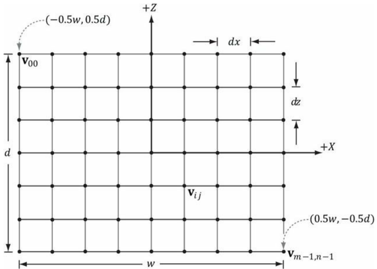
Figure 6.9. Grid construction.
