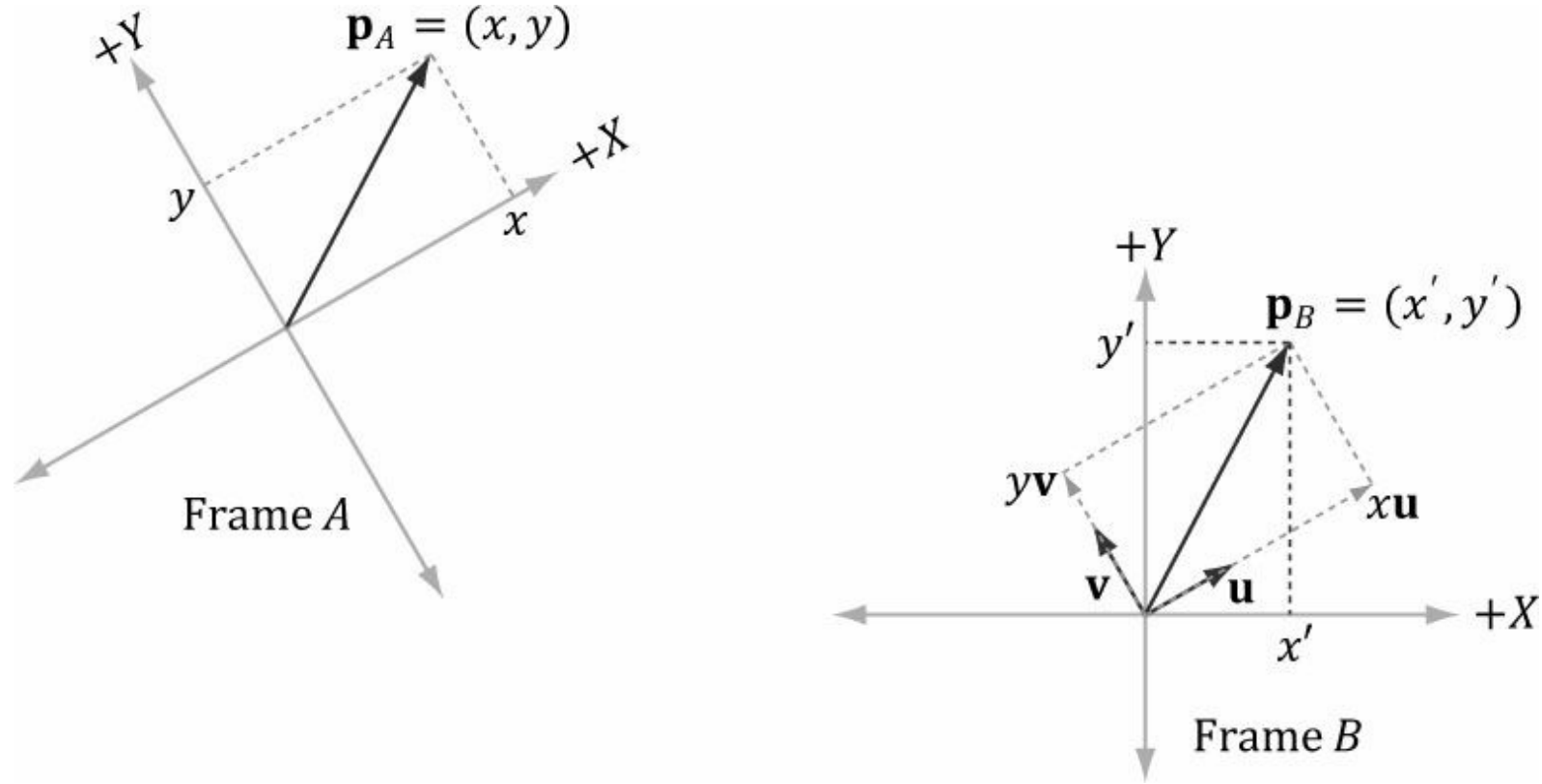
Figure 3.11. The geometry of finding the coordinates of \mathbf{p} relative to frame B .
