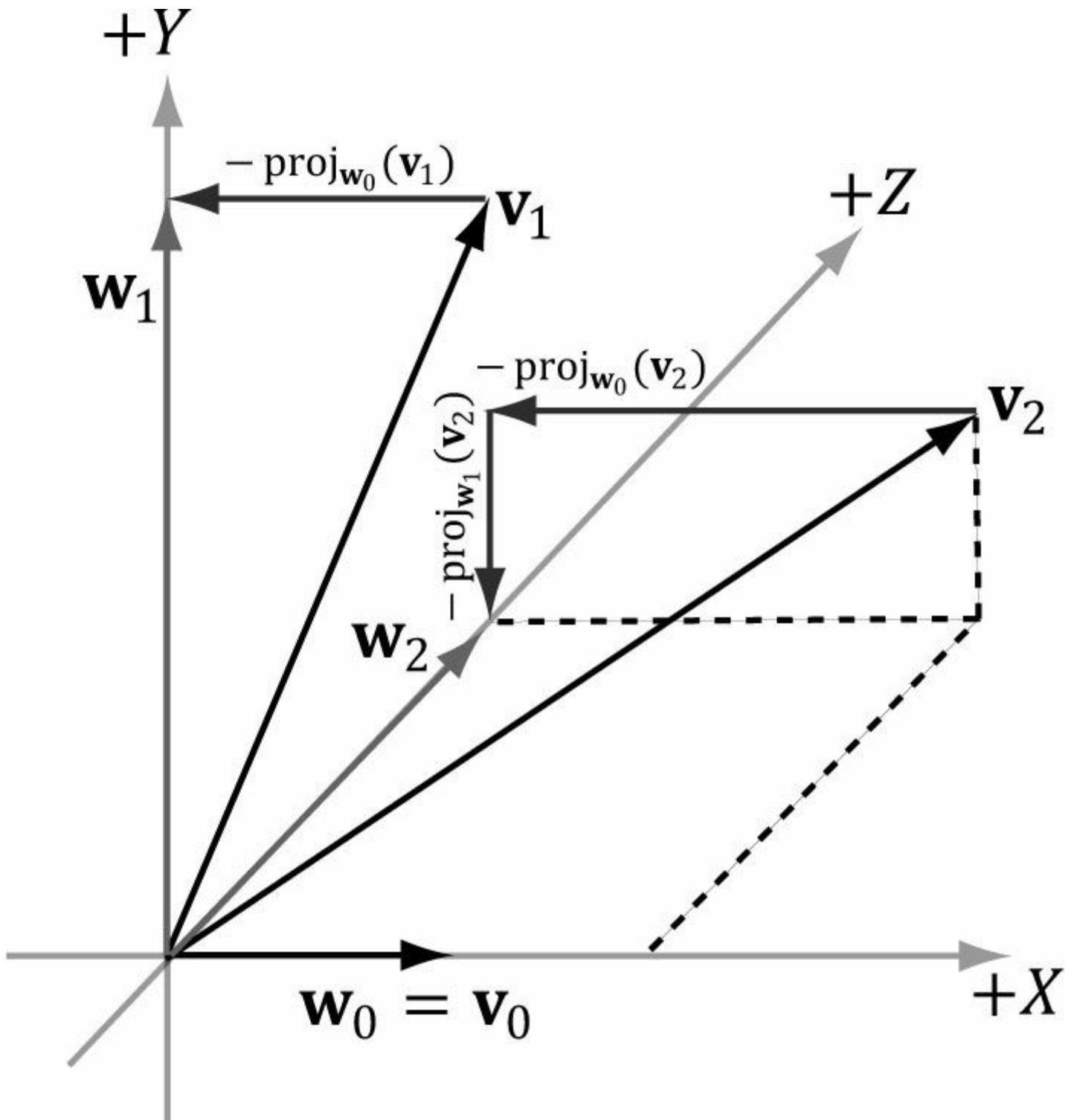
Figure 1.12. 3D orthogonalization.
