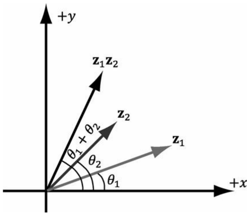
Figure 24.4. \mathbf{z}_1 = r_1(\cos \theta_1 + i \sin \theta_1) , \mathbf{z}_2 = (\cos \theta_2 + i \sin \theta_2) . The product \mathbf{z}_1 \mathbf{z}_2 rotates \mathbf{z}_1 by the angle \theta_2 .
