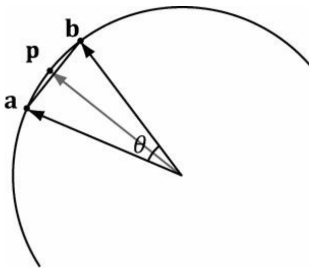
Figure 24.7. For small angles \theta between a and b , linear interpolation is a good approximation for spherical interpolation. However, when using linear interpolation, the interpolated quaternion no longer lies on the unit sphere, so you must normalize the result to project it back on to the unit sphere.
