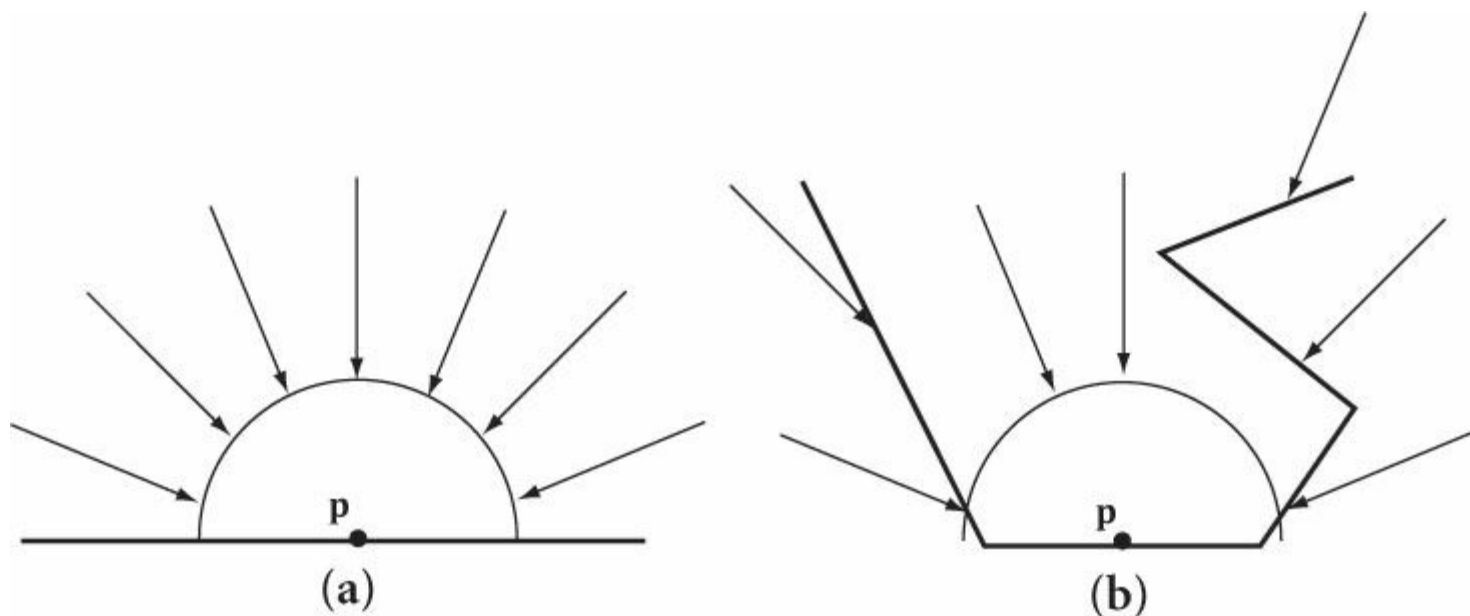
Figure 22.2. (a) A point p is completely unoccluded and all incoming light over the hemisphere about p reaches p . (b) Geometry partially occludes p and blocks incoming light rays over the hemisphere about p .
