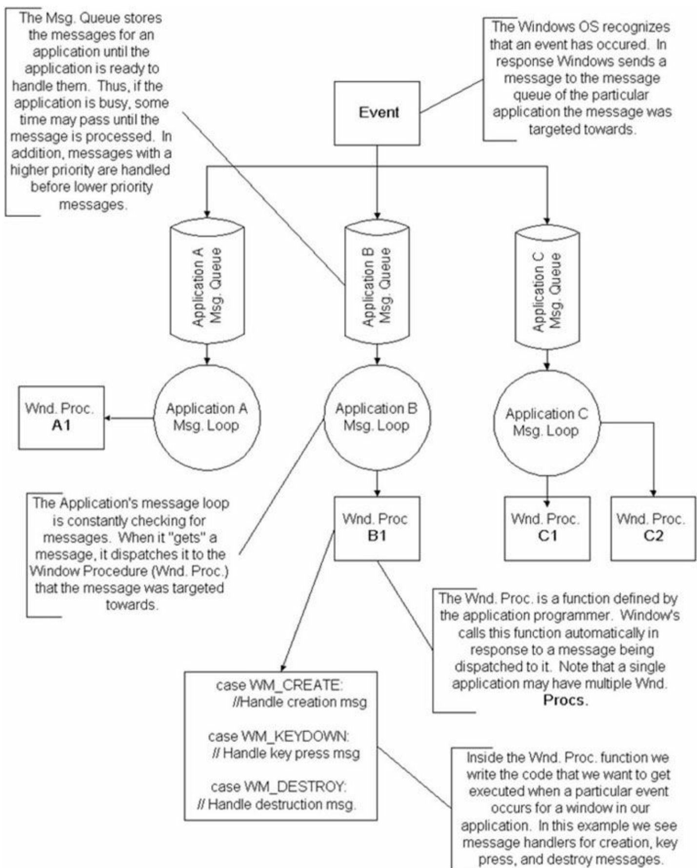
Figure A.1. The event driven programming model.
