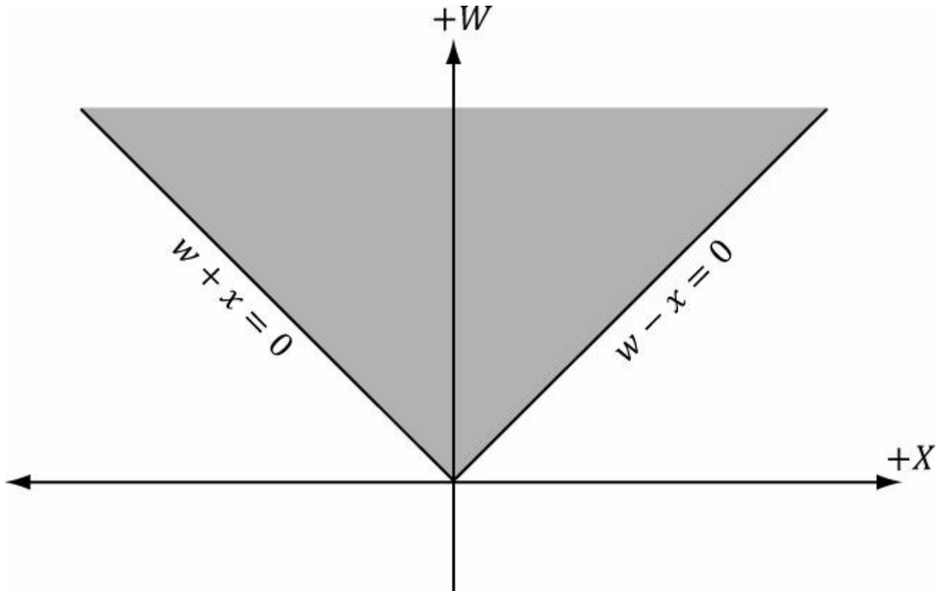
Figure 5.29. The frustum boundaries in the xw -plane in homogeneous clip space.
