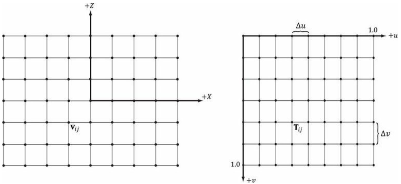
Figure 8.16. The texture coordinates of the grid vertex v_{ij} in xz -space are given by the ij th grid vertex T_{ij} in uv -space.
