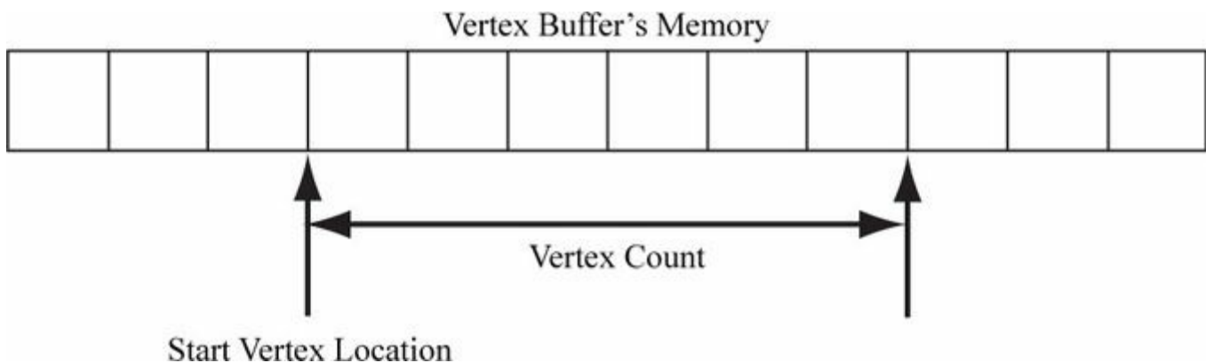
Figure 6.2. StartVertexLocation specifies the index (zero-based) of the first vertex in the vertex buffer to begin drawing. VertexCount specifies the number of vertices to draw.
