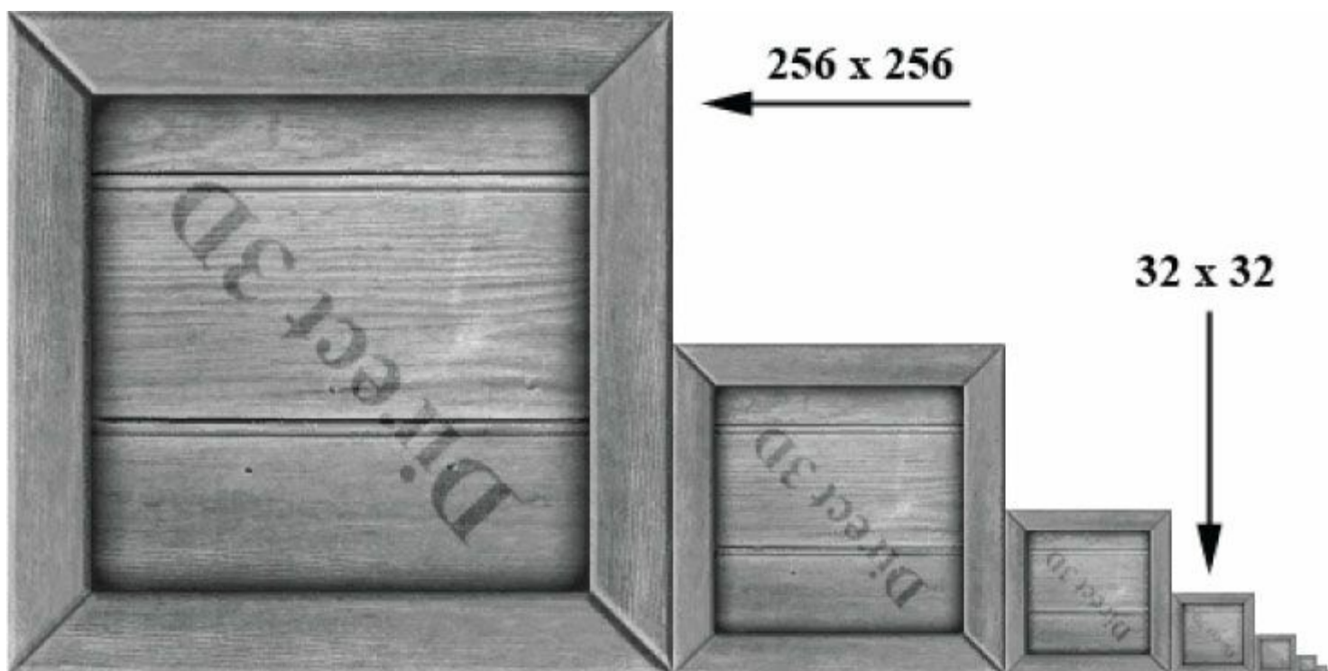
Figure 8.8. A chain of mipmaps; each successive mipmap is half the size, in each dimension, of the previous mipmap level of detail down to 1 \times 1 .
