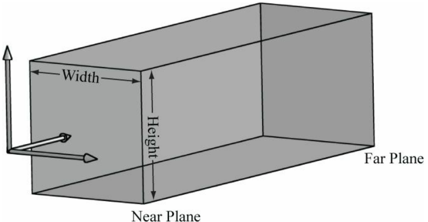
Figure 21.1. The orthographic viewing volume is a box that is axis aligned with the view coordinate system.
