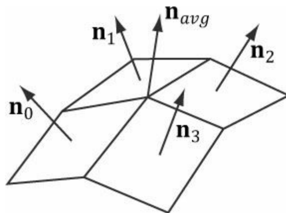
Figure 7.6. The middle vertex is shared by the neighboring four polygons, so we approximate the middle vertex normal by averaging the four polygon face normals.
