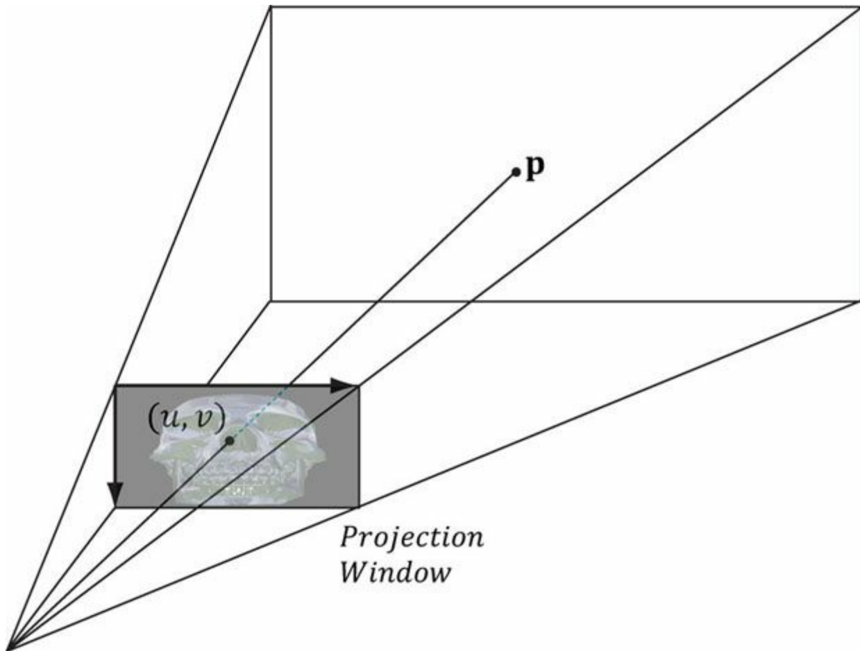
Figure 21.4. The texel identified by the coordinates (u, v) relative to the texture space on the projection window is projected onto the point p by following the line of sight from the light origin to the point p .
