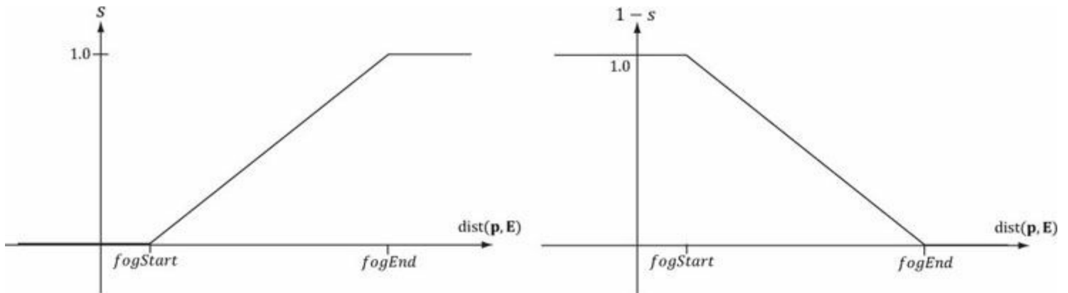
Figure 9.13. (Left) A plot of s (the fog color weight) as a function of distance. (Right) A plot of 1 - s (the lit color weight) as a function of distance. As s increases, (1 - s) decreases the same amount.
