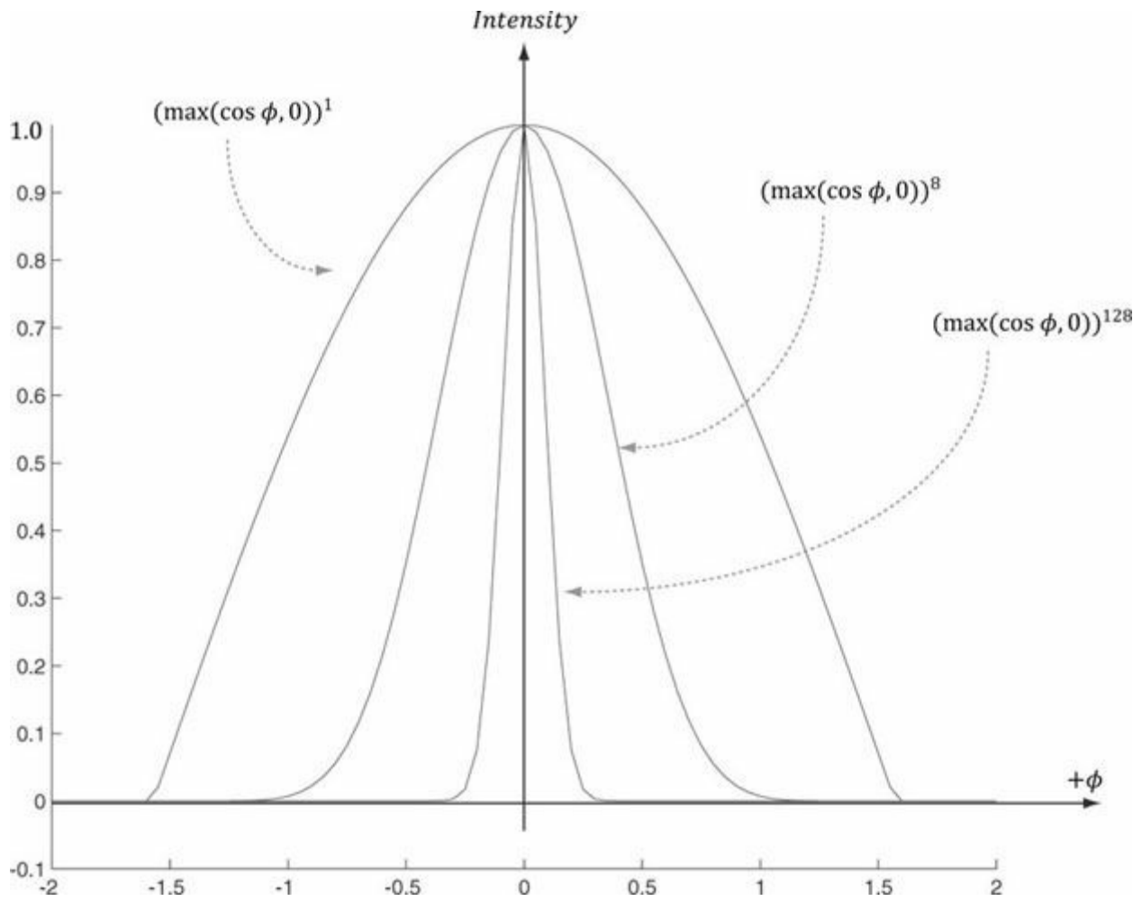
Figure 7.12. Plots of the cosine functions with different powers of p \geq 1 .
