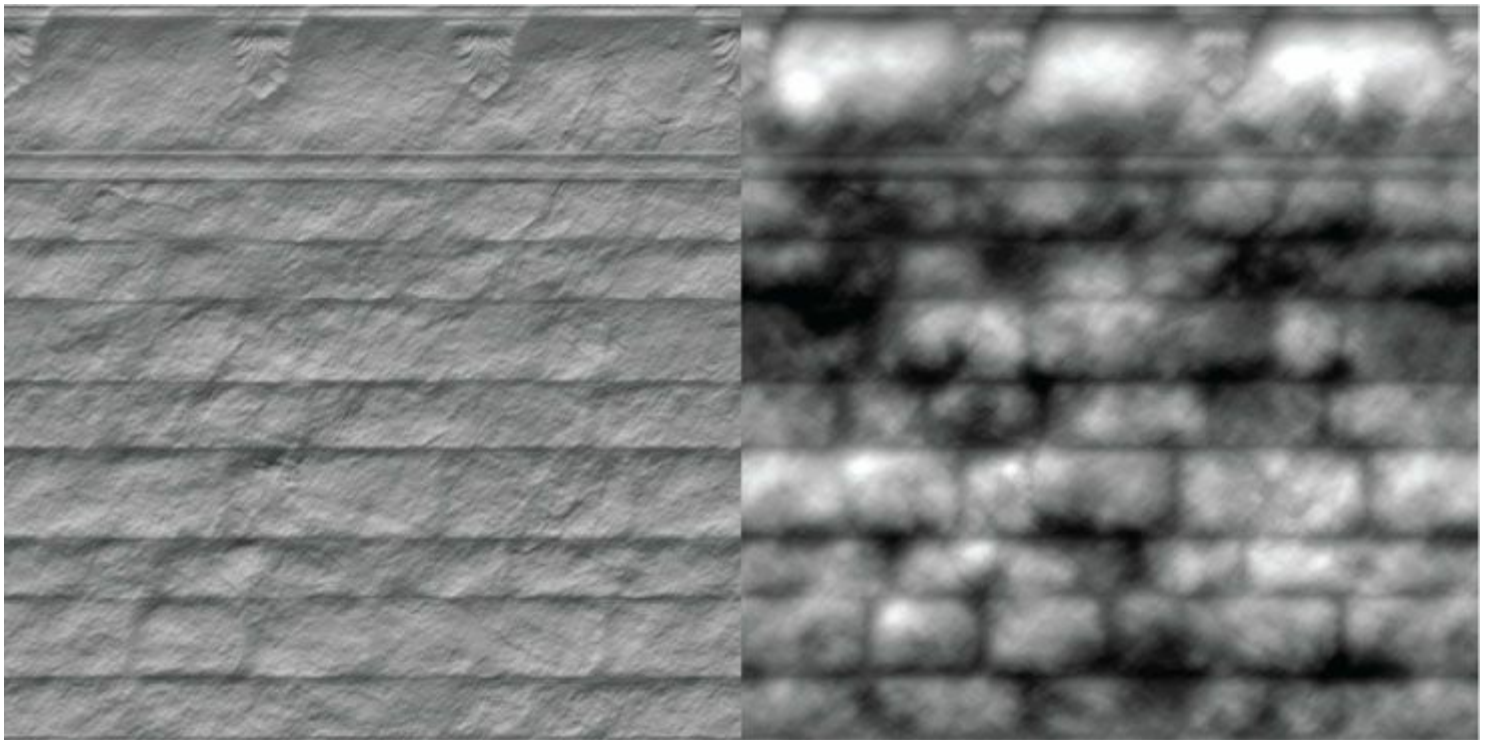
Figure 18.9. (Left) Normal map. (Right) Heightmap stored in the alpha channel of the normal map. A white value represents the highest height, and a black value represents the lowest height. Gray values represent intermediate heights.
