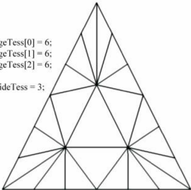
Figure 13.3. Triangle subdivisions based on edge and interior tessellation factors.
