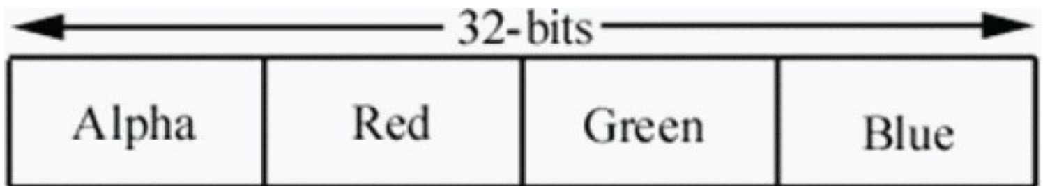
Figure 5.10. A 32-bit color, where a byte is allocated for each color component alpha, red, green, and blue.
