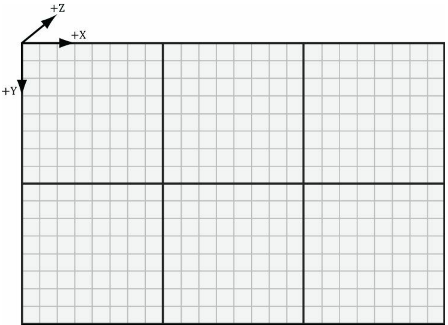
Figure 12.3. Dispatching a grid of 3 \times 2 thread groups. Each thread group has 8 \times 8 threads.
