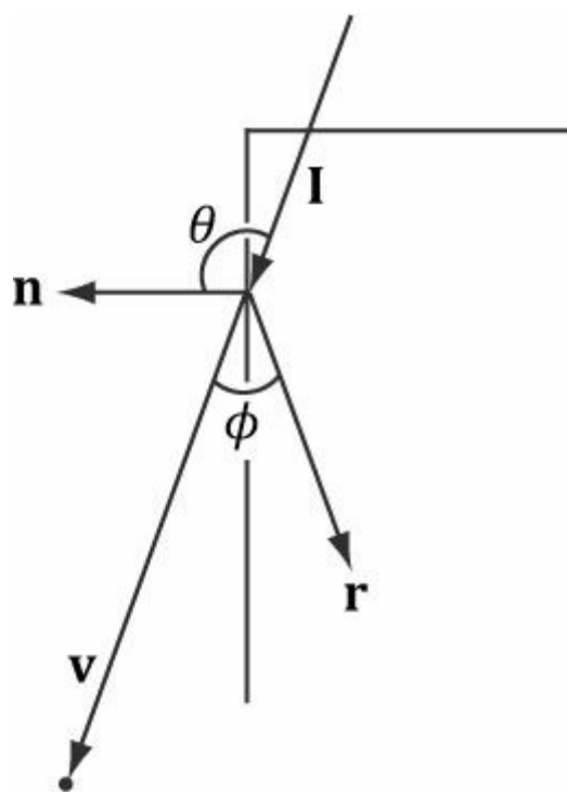
Figure 7.13. The eye can receive specular light even though the light strikes the back of a surface. This is incorrect, so we must detect this situation and set k_s = 0 in this case.
