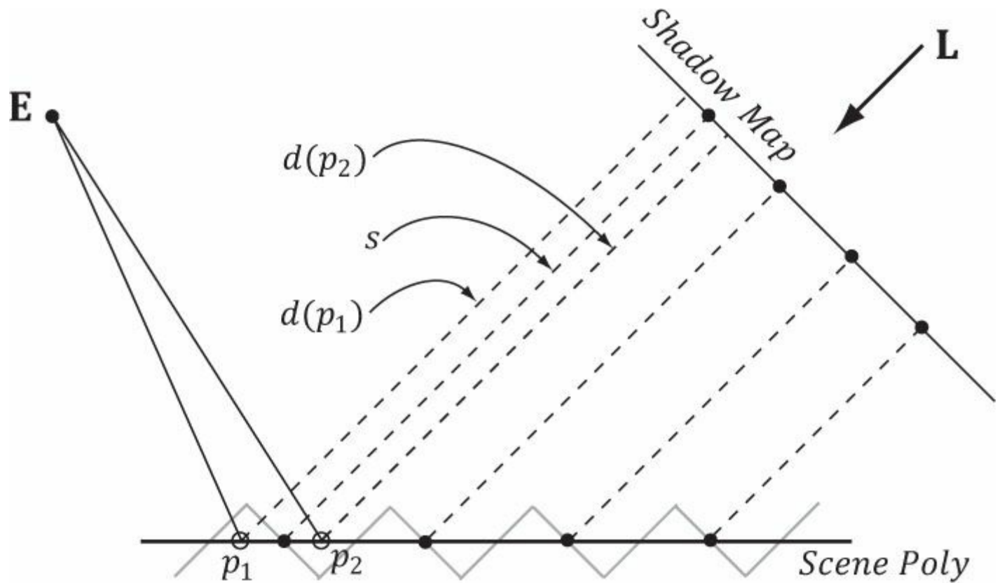
Figure 21.8. The shadow map samples the depth of the scene. Observe that due to finite resolution of the shadow map, each shadow map texel corresponds to an area of the scene. The eye E sees two points on the scene p_1 and p_2 that correspond to different screen pixels. However, from the viewpoint of the light, both points are covered by the same shadow map texel (that is, s(p_1) = s(p_2) = s ). When we do the shadow map test, we have d(p_1) > s and d(p_2) \leq s . Thus, p_1 will be colored as if it were in shadow, and p_2 will be colored as if it were not in shadow. This causes the shadow acne.
