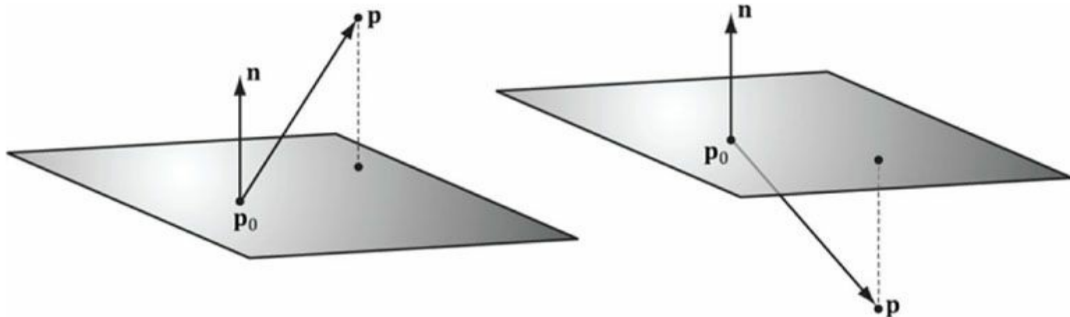
Figure C.8. Point/plane spatial relation.
