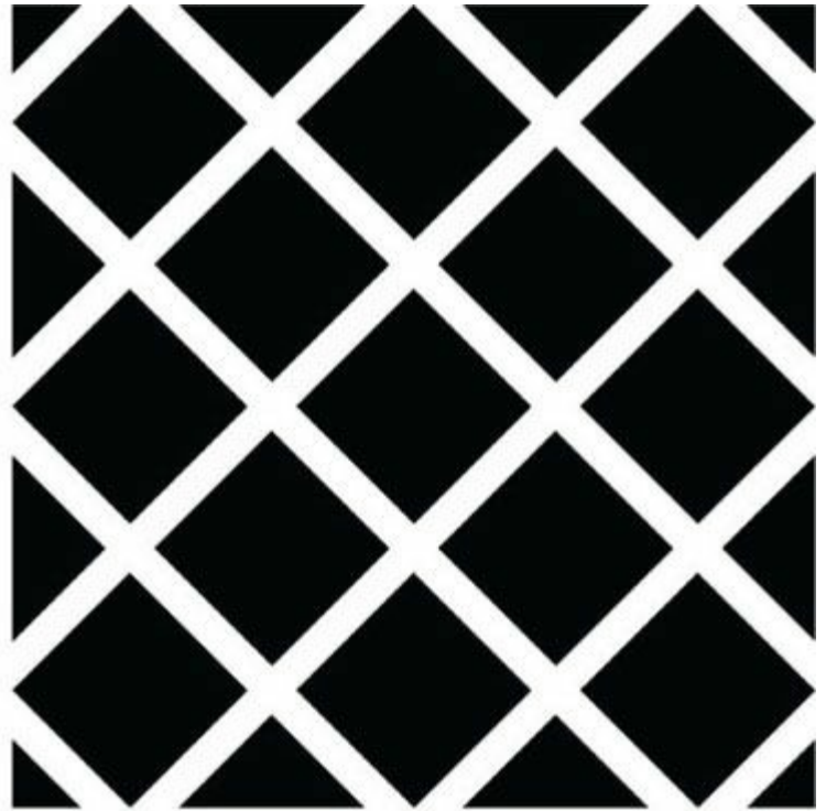
Alpha Channel
