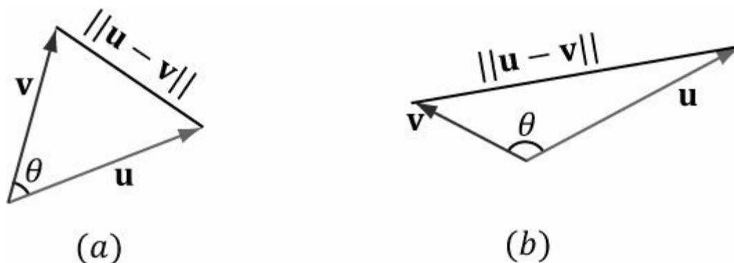
Figure 1.9. In the left figure, the angle \theta between \mathbf{u} and \mathbf{v} is an acute angle. In the right figure, the angle \theta between \mathbf{u} and \mathbf{v} is an obtuse angle. When we refer to the angle between two vectors, we always mean the smallest angle, that is, the angle \theta such that 0 \leq \theta \leq \pi .
