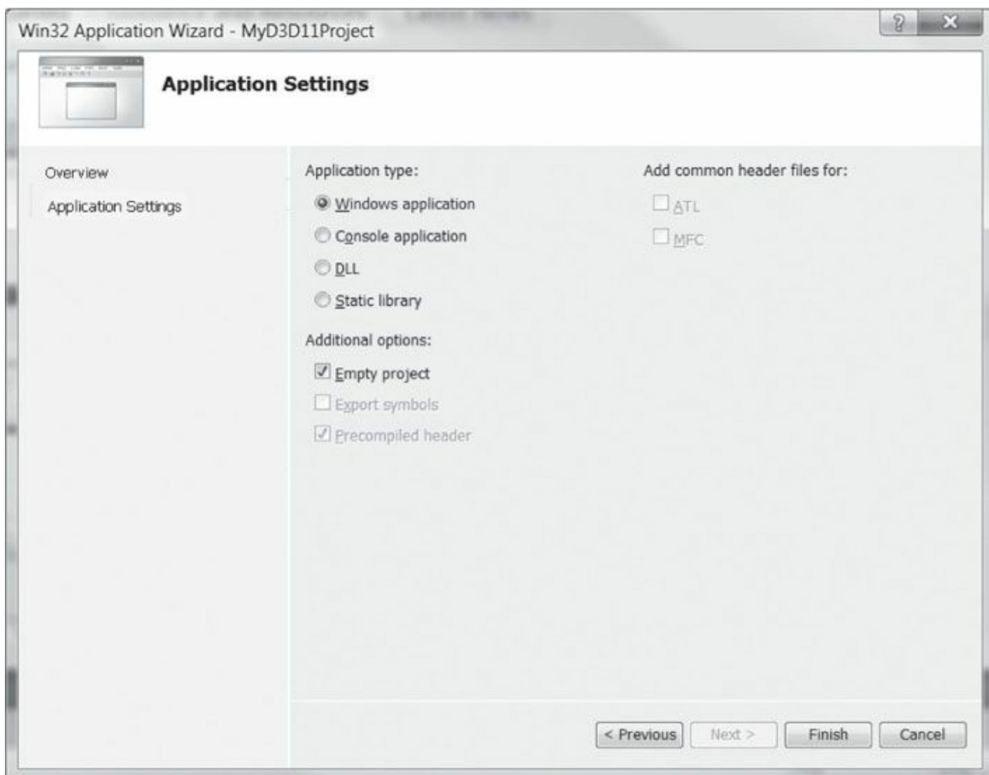
Figure 5. Application settings.
