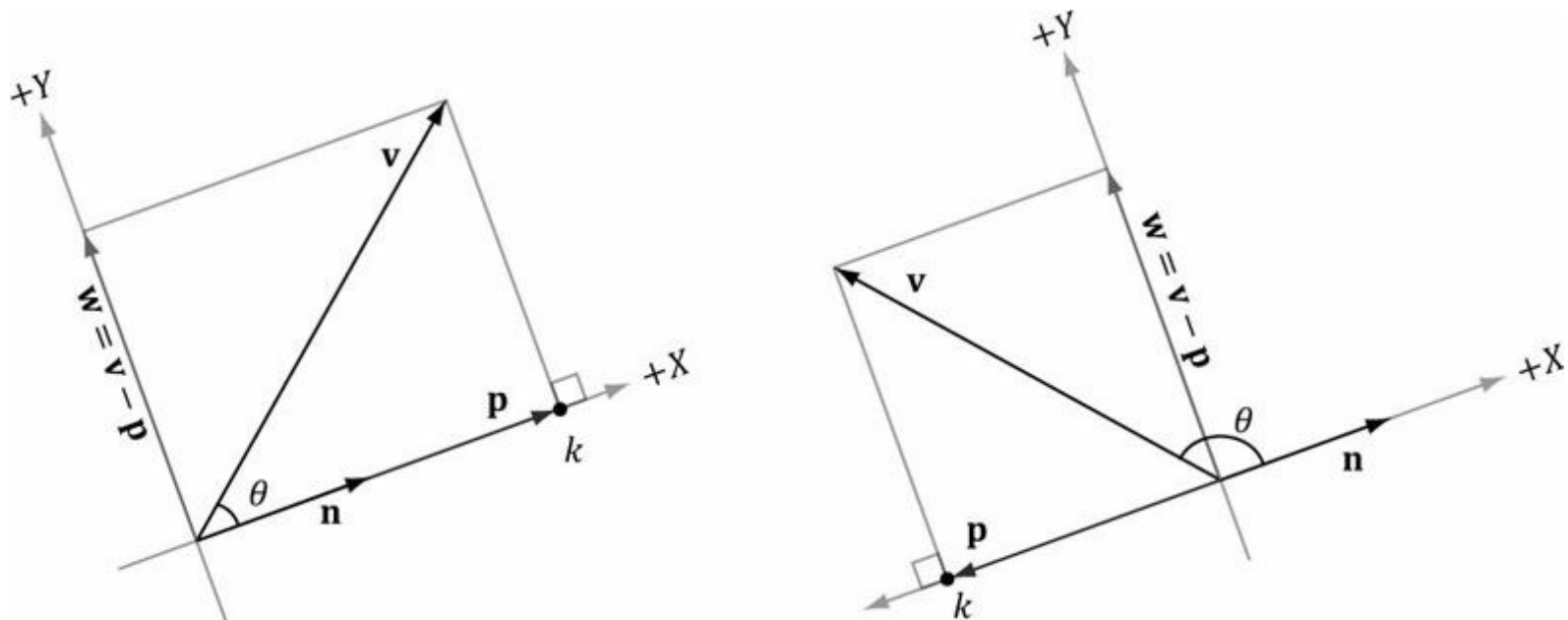
Figure 1.10. The orthogonal projection of \mathbf{v} on \mathbf{n} .
