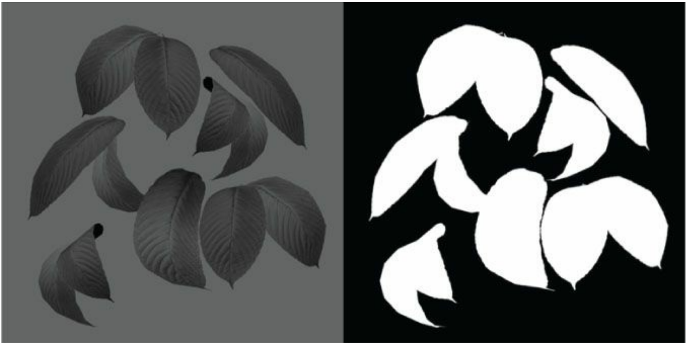
Figure 21.14. Leaf texture.
