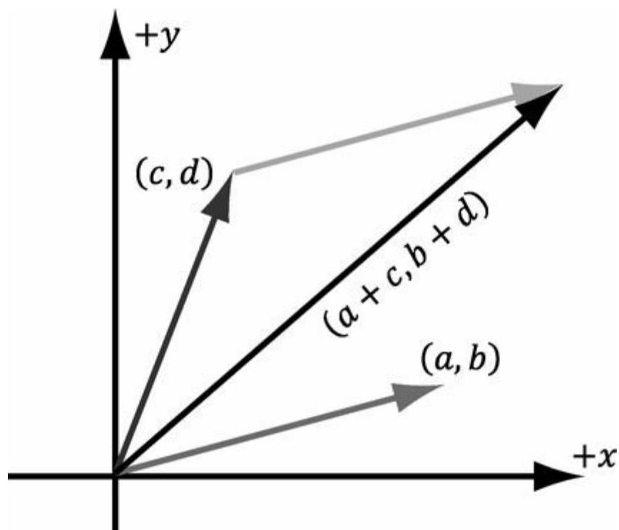
Figure 24.1. Complex addition is reminiscent of vector addition in the plane.
