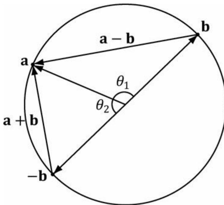
Figure 24.10. Interpolating from \mathbf{a} to \mathbf{b} results in interpolating over the larger arc \theta_1 on the 4D unit sphere, whereas interpolating from \mathbf{a} to -\mathbf{b} results in interpolating over the shorter arc \theta_2 on the 4D unit sphere. We want to choose the shortest arc on the 4D unit sphere.
