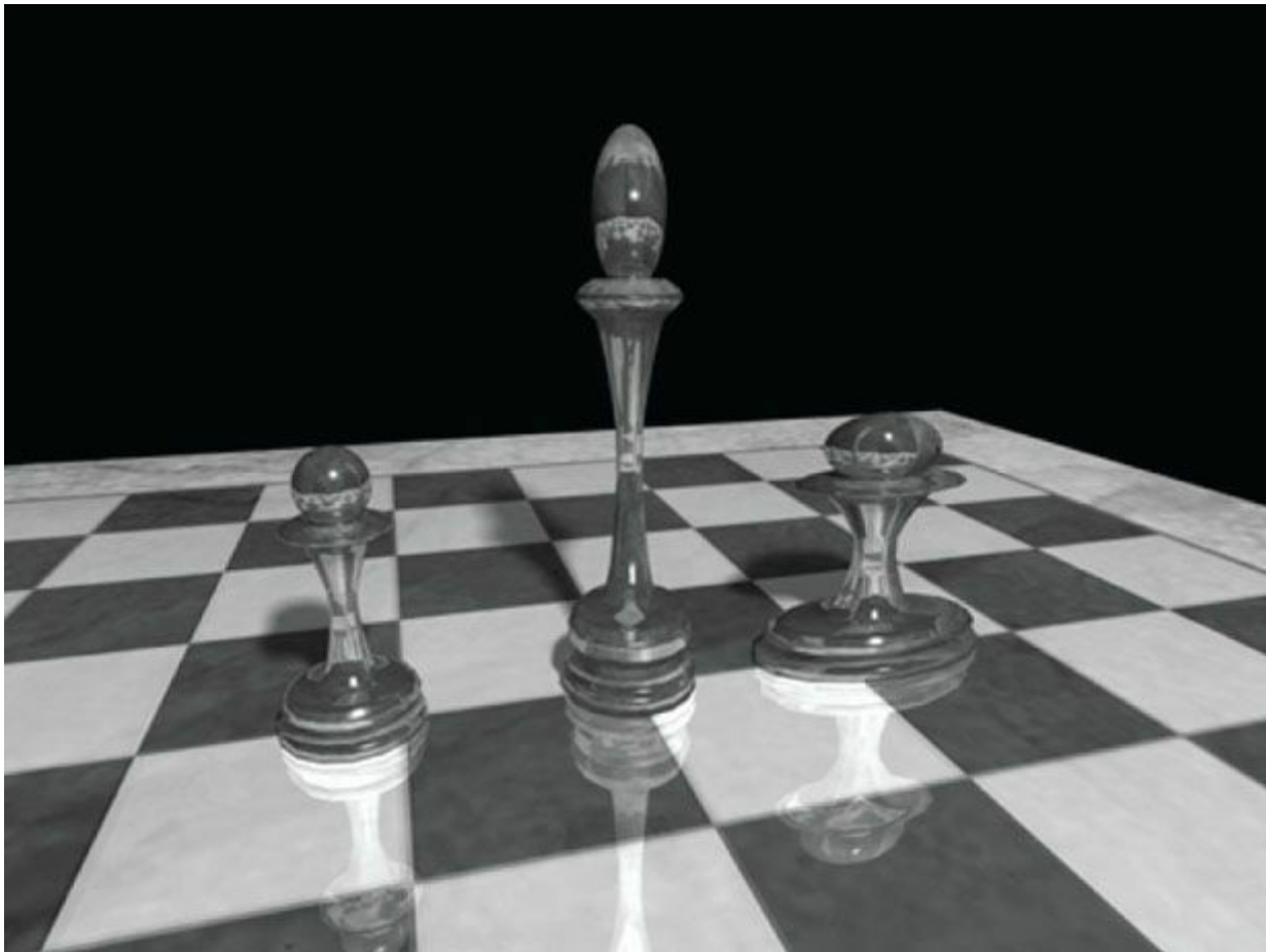
Figure 3.1. The left pawn is the original object. The middle pawn is the original pawn scaled 2 units on the y -axis making it taller. The right pawn is the original pawn scaled 2 units on the x -axis making it fatter.
