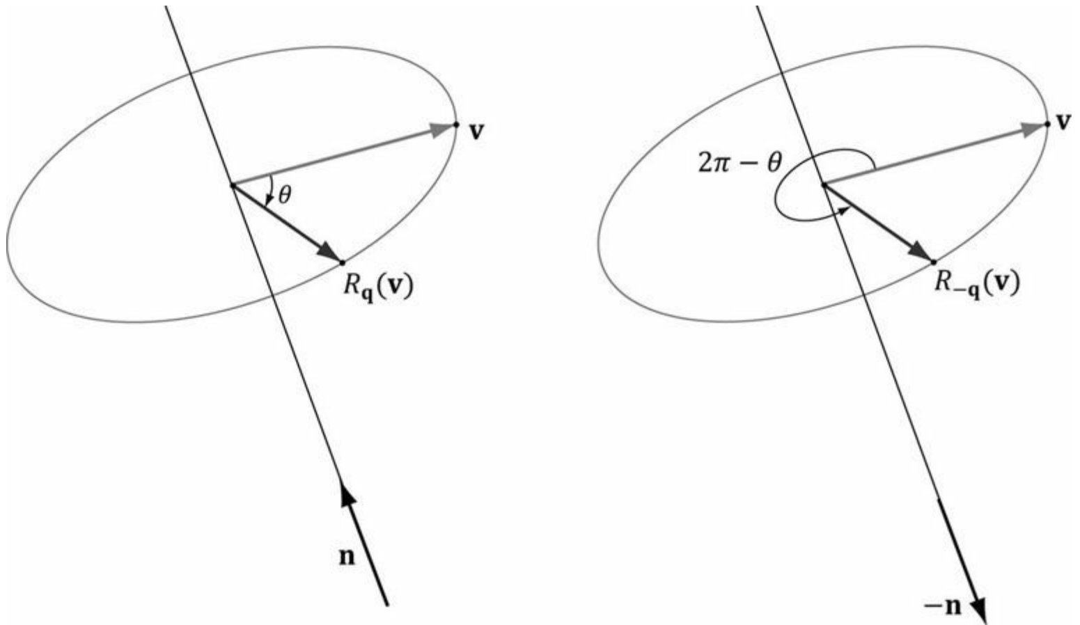
Figure 24.9. R_{\mathbf{q}} rotates \theta about the axis \mathbf{n} , and R_{-\mathbf{q}} rotates 2\pi - \theta about the axis -\mathbf{n} .
