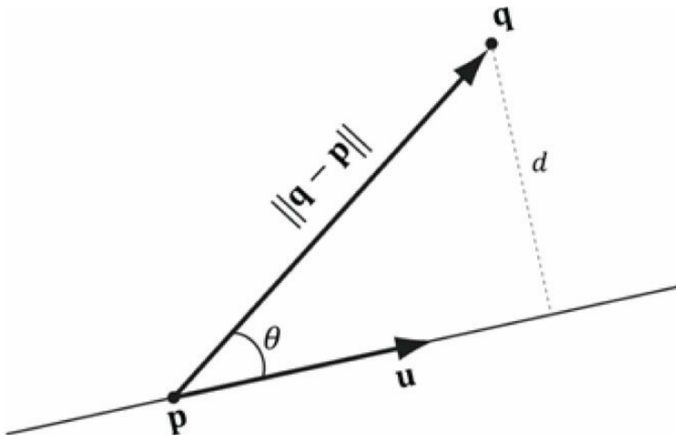
Figure C.12. Distance from \mathbf{q} to the line.
