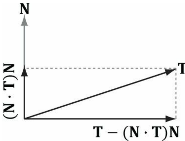
Figure 18.6. Since \|N\| = 1 , \text{proj}_N(T) = (T \cdot N)N . The vector T - \text{proj}_N(T) is the portion of T orthogonal to N .
