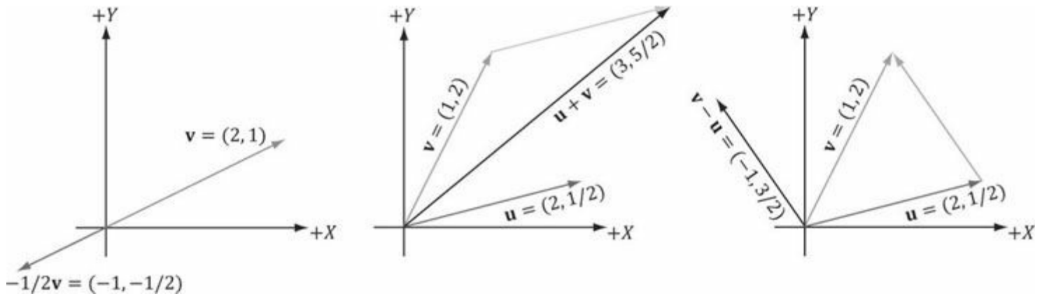
Figure 1.6. (a) The geometric interpretation of scalar multiplication. (b) The geometric interpretation of vector addition. (c) The geometric interpretation of vector subtraction.
