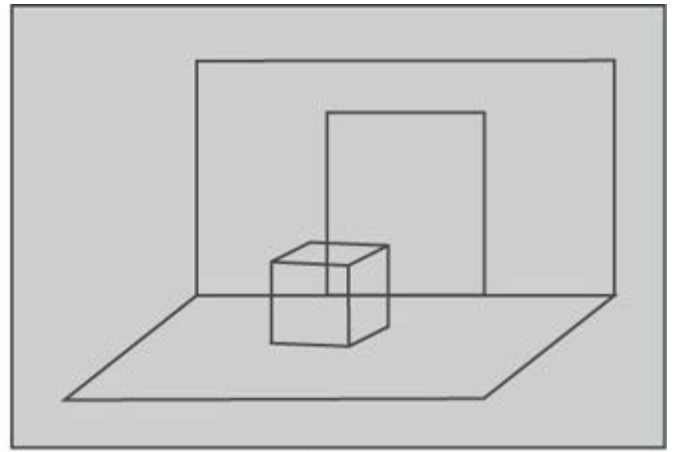
Stencil buffer
