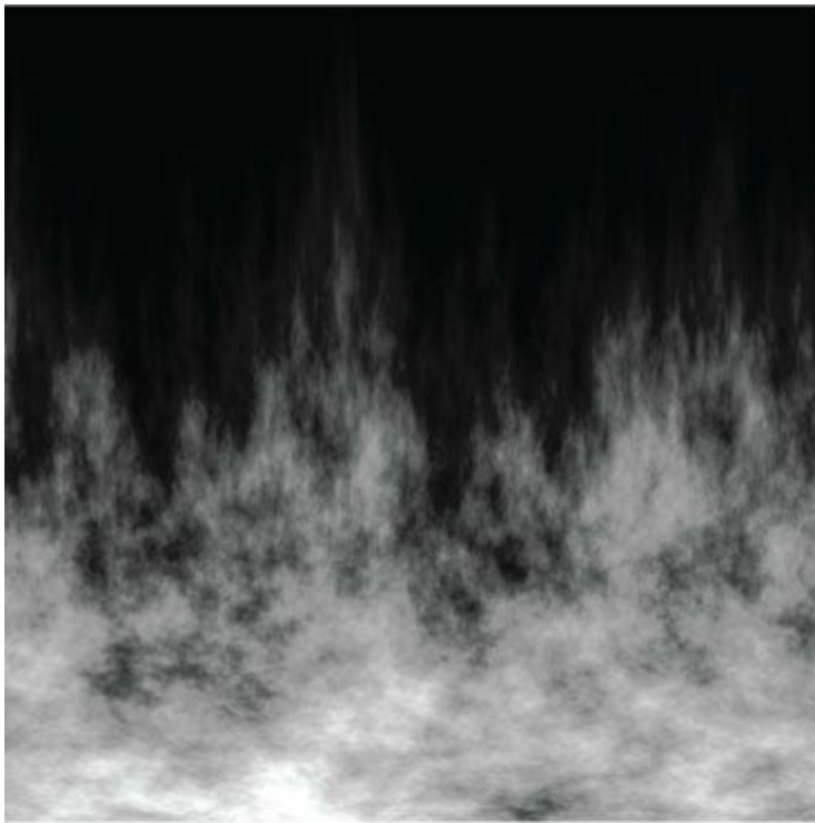
RGB Channels
