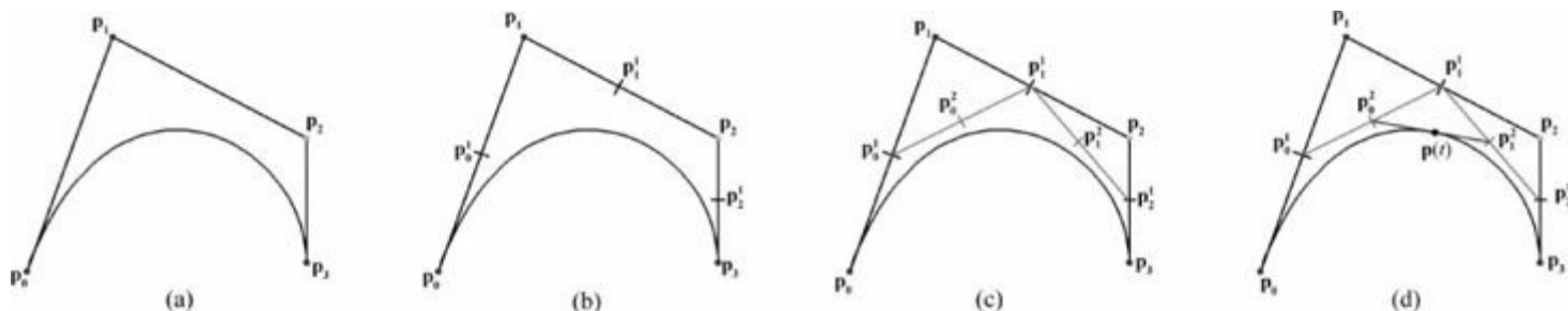
Figure 13.6. Repeated linear interpolation defined points on the cubic Bézier curve. The figure uses t = 0.5 . (a) The 4 control points and the curve they define. (b) Linearly interpolate between the control points to calculate the first generation of intermediate points. (c) Linearly interpolate between the first generation intermediate points to get the second generation intermediate points. (d) Linearly interpolate between the second generation intermediate points to get the point on the curve.
