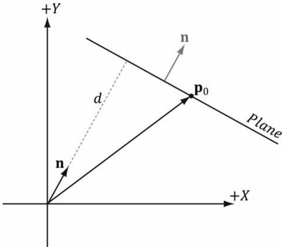
Figure C.6. A plane defined by a normal vector \mathbf{n} and a point \mathbf{p}_0 on the plane. If \mathbf{p}_0 is a point on the plane, then the point \mathbf{p} is also on the plane if and only if the vector \mathbf{p} - \mathbf{p}_0 is orthogonal to the plane's normal vector.
