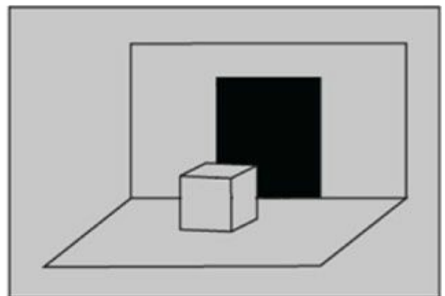
Stencil Buffer
