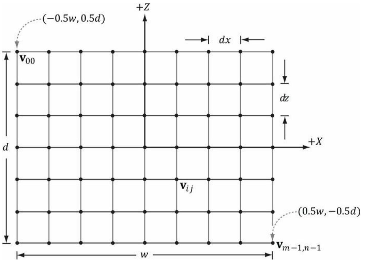
Figure 19.4. Grid properties.
