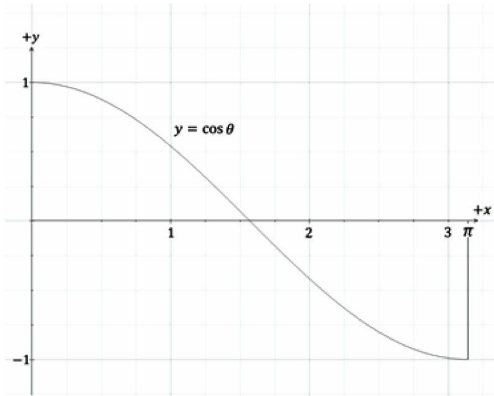
Figure 24.5. For a number y \in [-1, 1] there exists an angle \theta such that y = \cos \theta
