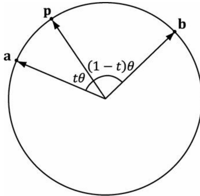
Figure 24.6. Interpolating along the 4D unit sphere from \mathbf{a} to \mathbf{b} by an angle t\theta . The angle between \mathbf{a} and \mathbf{b} is \theta , the angle between \mathbf{a} and \mathbf{p} is t\theta , and the angle between \mathbf{p} and \mathbf{b} is (1-t)\theta .
