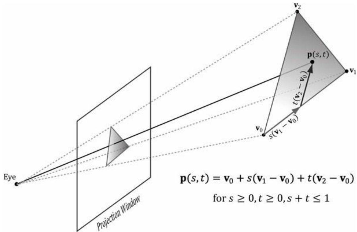
Figure 5.33. An attribute value p(s, t) on a triangle can be obtained by linearly interpolating between the attribute values at the vertices of the triangle.
