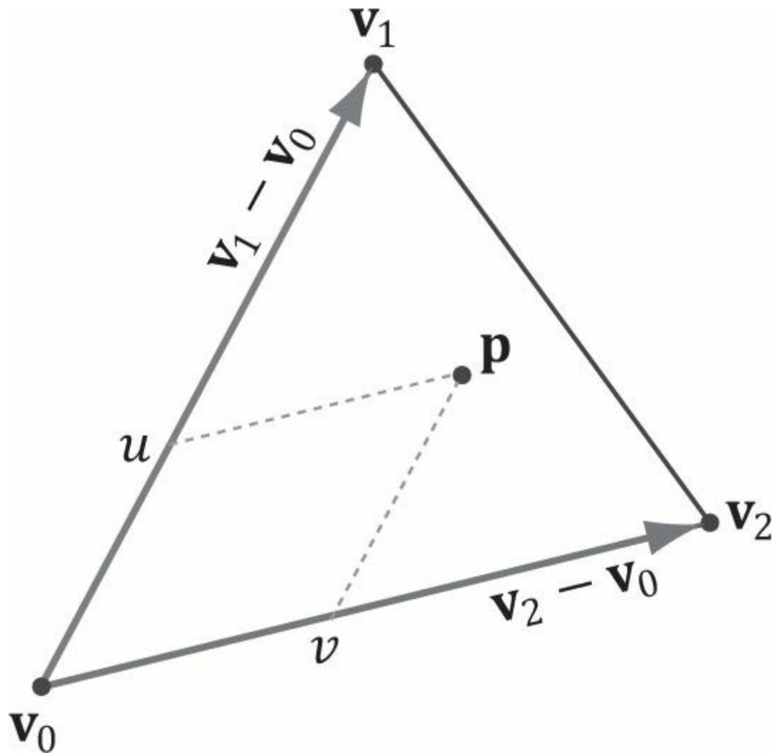
Figure 16.5. The point p in the plane of the triangle has coordinates (u, v) relative to the skewed coordinate system with origin v_0 and axes v_1 - v_0 and v_2 - v_0 .
