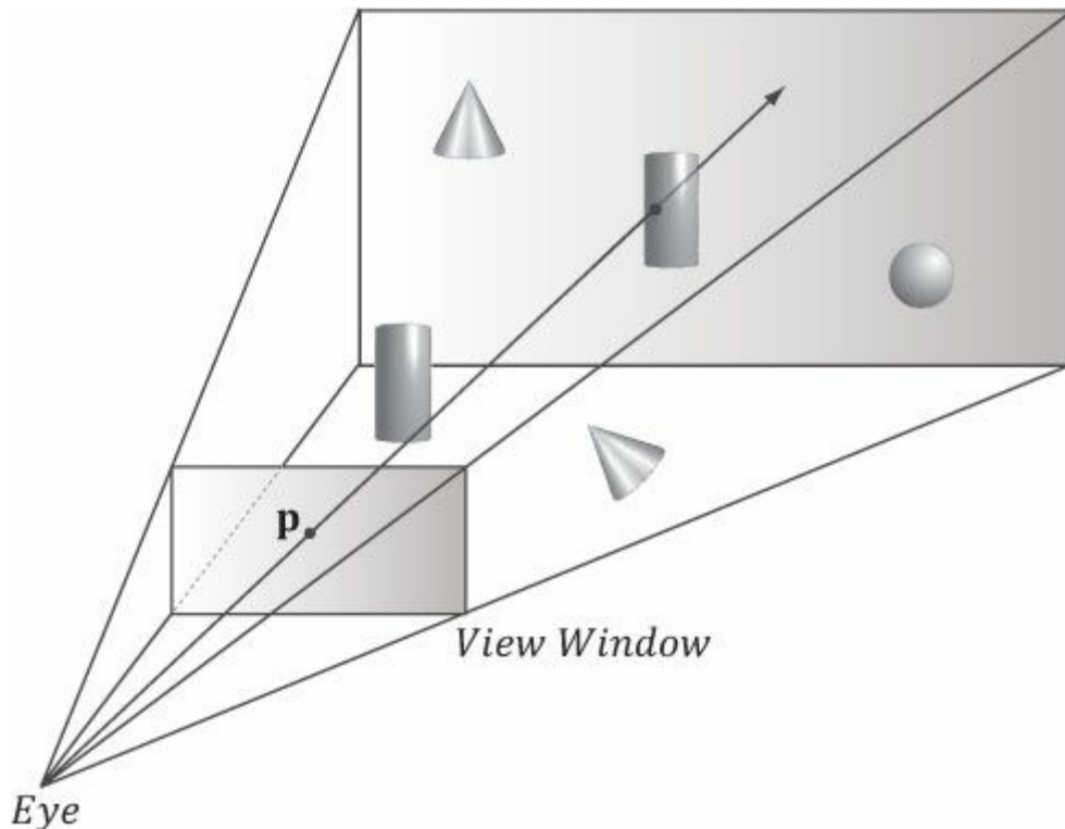
Figure 16.3. A ray shooting through p will intersect the object whose projection surrounds p . Note that the projected point p on the projection window corresponds to the clicked screen point s .
