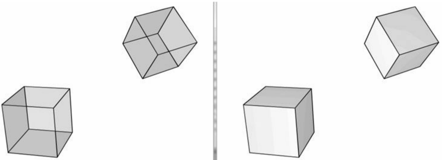
Figure 5.32. (Left) We draw the cubes with transparency so that you can see all six sides. (Right) We draw the cubes as solid blocks. Note that we do not see the three back-facing sides because the three front-facing sides occlude them—thus the back-facing triangles can actually be discarded from further processing and no one will notice.
