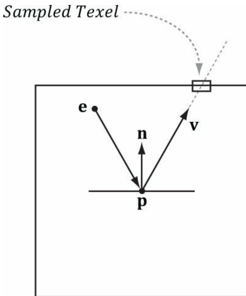
Figure 17.7. Here e is the eye point, and n is the surface normal at the point p . The texel that gets mapped to a point p on the surface is given by the reflection vector v (i.e., we use v as the lookup vector), which is the reflection of the vector from e to p about the surface. In this way, the eye sees the reflected environment.
