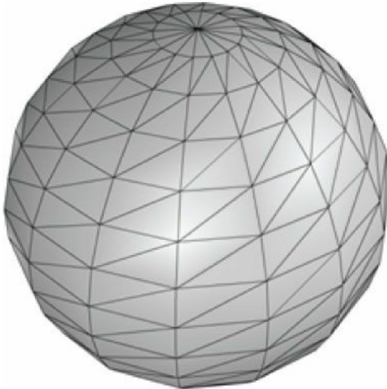
Figure 6.15. The idea of slices and stacks also apply to a sphere to control the level of tessellation.
