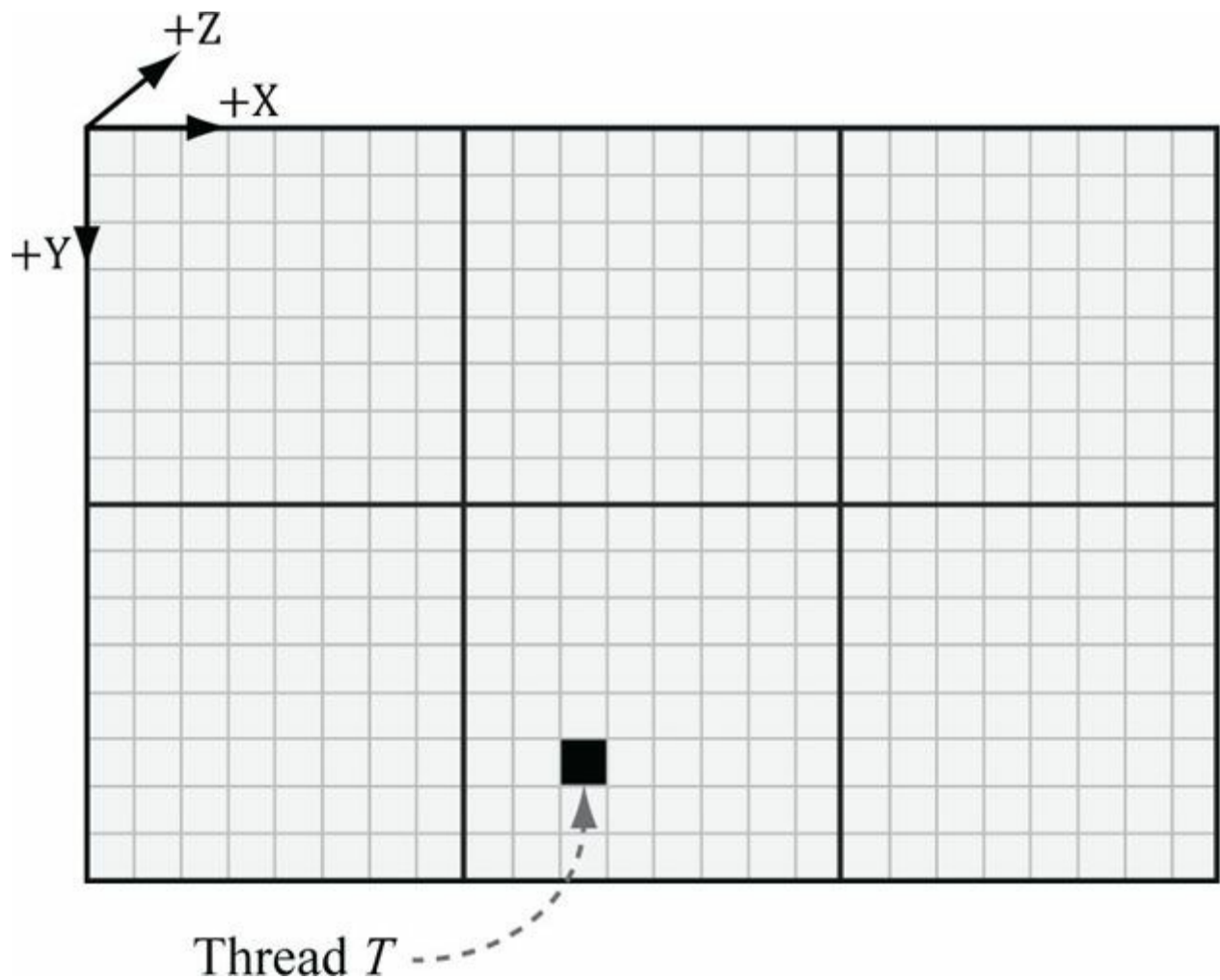
Figure 12.4. Consider the marked thread T . Thread T has thread group ID (1, 1, 0) . It has group thread ID (2, 5, 0) . It has dispatch thread ID (1, 1, 0) \otimes (8, 8, 0) + (2, 5, 0) = (10, 13, 0) . It has group index ID 5 \cdot 8 + 2 = 42 .
