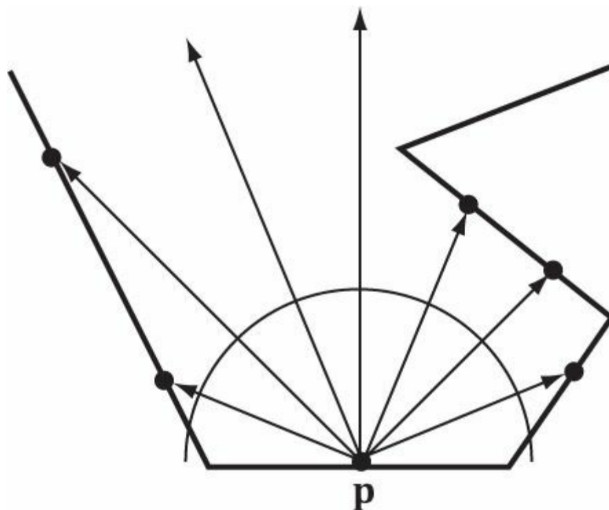
Figure 22.3. Estimating ambient occlusion via ray casting.
