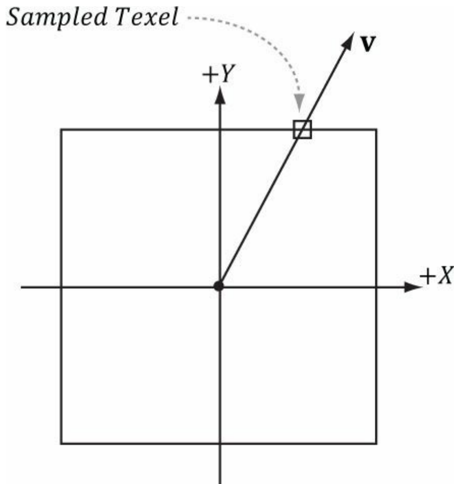
Figure 17.1. We illustrate in 2D for simplicity; in 3D the square becomes a cube. The square denotes the cube map centered and axis-aligned with some coordinate system. We shoot a vector v from the origin. The texel v intersects is the sampled texel. In this illustration, v intersects the cube face corresponding to the +Y axis.
