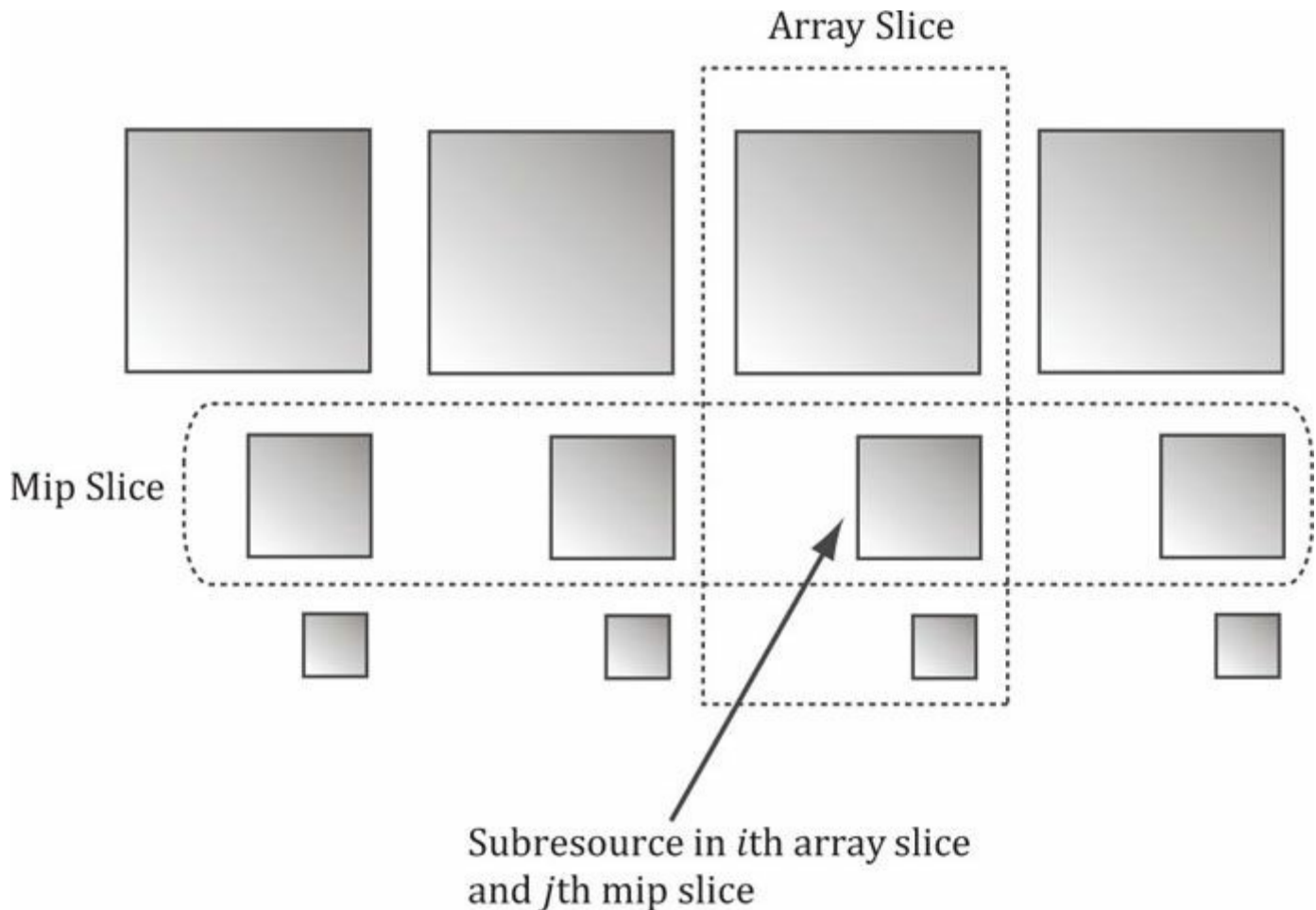
Figure 11.8. A texture array with four textures. Each texture has three mipmap levels.
