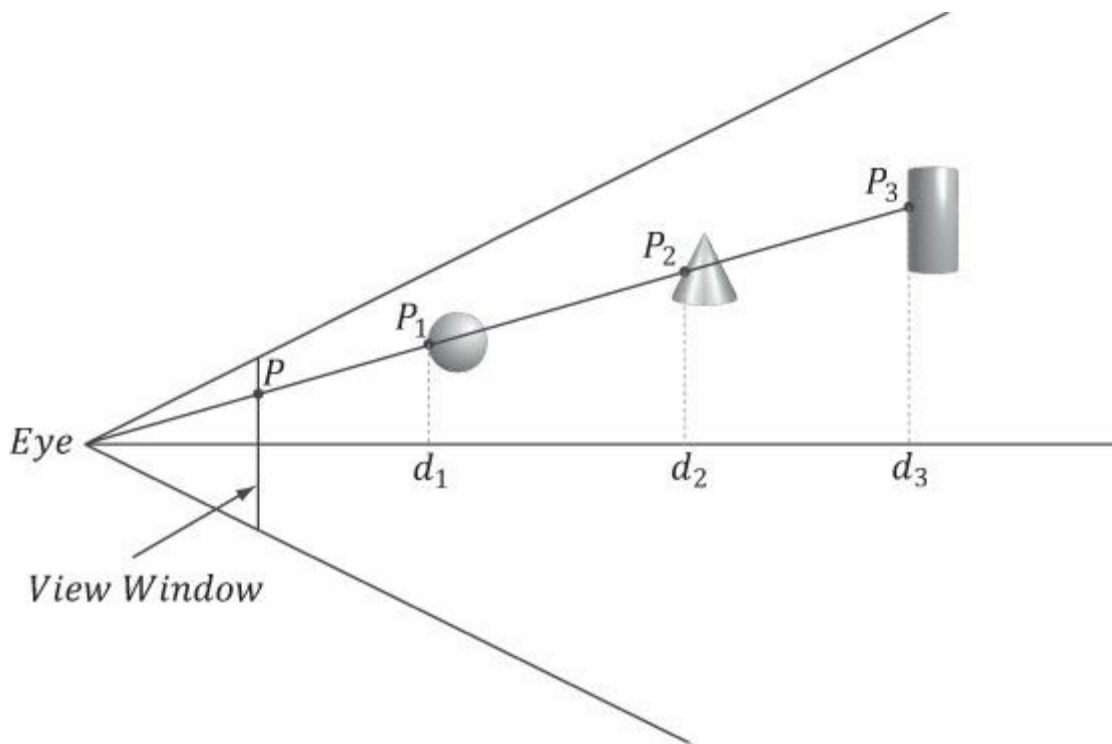
Figure 16.2. A side view of the frustum. Observe that several points in 3D space can get projected onto a point on the projection window.
