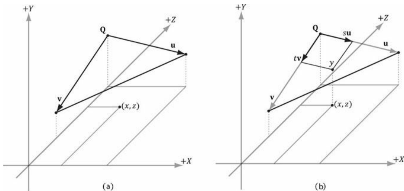
Figure 19.14. (a) Computing two vectors on the upper-triangle edges. (b) The height is the y -coordinate of the vector.
