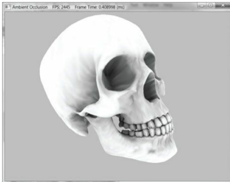
Figure 22.4. The mesh is rendered only with ambient occlusion—there are no scene lights. Notice how the crevices are darker; this is because when we cast rays out they are more likely to intersect geometry and contribute to occlusion. On the other hand, the skull cap is white (unoccluded) because when we cast rays out over the hemisphere for points on the skull cap, they will not intersect any geometry of the skull.
