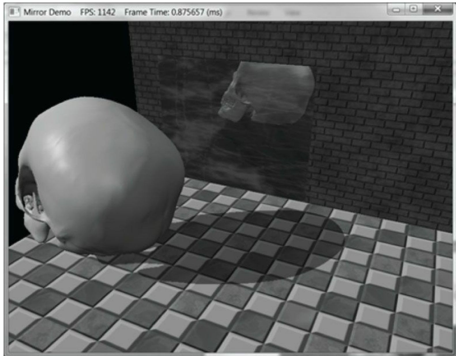
Figure 10.6. The main light source casts a planar shadow in the “Mirror” demo.
