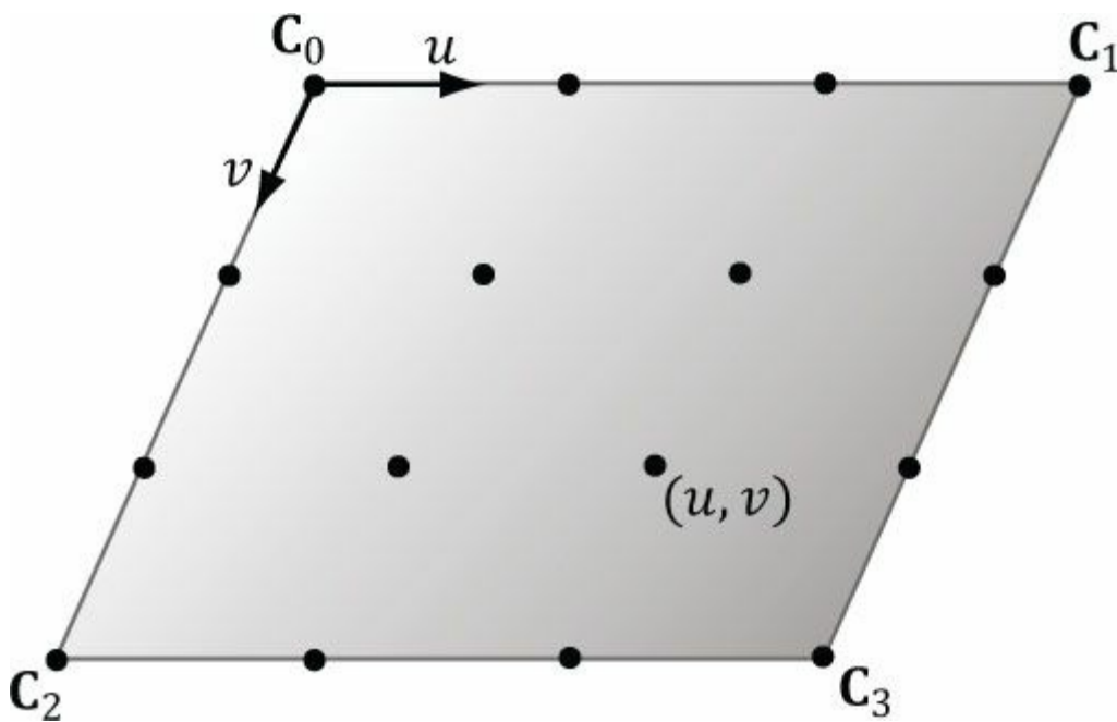
Figure 13.4. The tessellation of a quad patch with 4 control points generating 16 vertices in the normalized uv -space, with coordinates in [0, 1]^2 .
