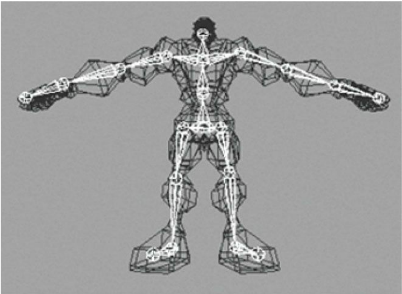
Figure 25.6. A character mesh. The highlighted bone chain represents the character's skeleton. The dark colored polygons represent the character's skin. The skin vertices are relative to the bind space , which is the coordinate system the mesh was modeled in.
