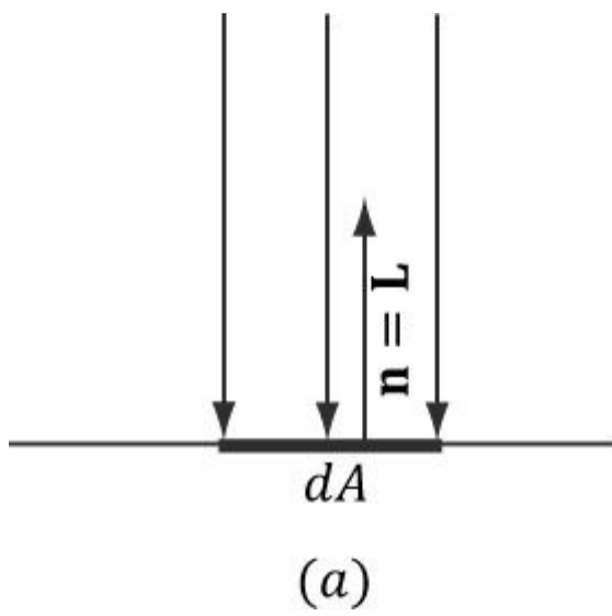
Figure 7.8. Consider a small area element dA . (a) The area dA receives the most light when the normal vector \mathbf{n} and light vector \mathbf{L} are aligned. (b) The area dA receives less light as the angle \theta between \mathbf{n} and \mathbf{L} increases (as depicted by the light rays that miss the surface dA ).
