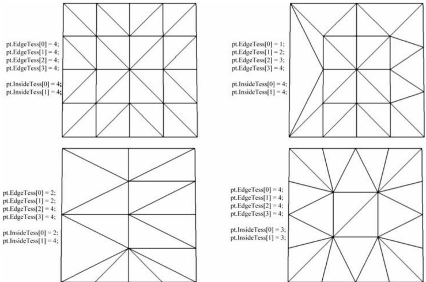
Figure 13.2. Quad subdivisions based on edge and interior tessellation factors.
