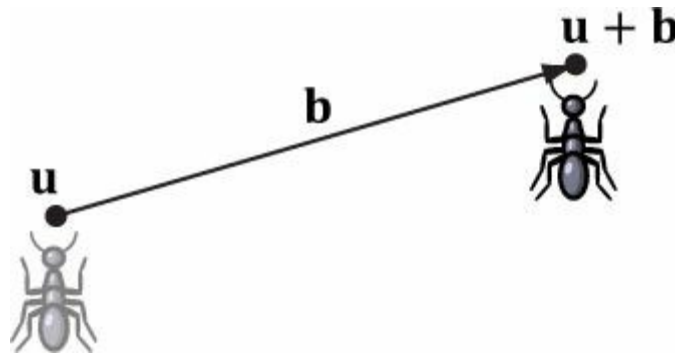
Figure 3.5. Displacing the position of the ant by some displacement vector \mathbf{b} .
