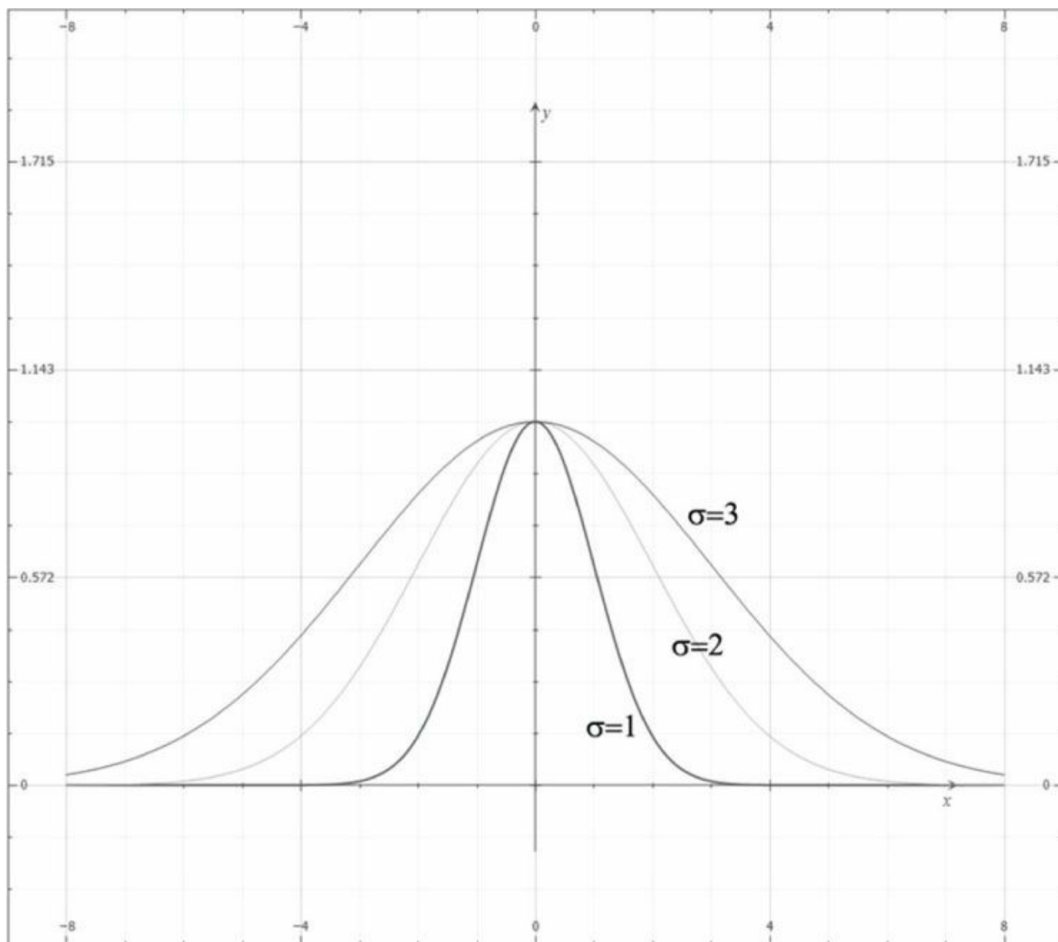
Figure 12.6. Plot of G(x) for \sigma = 1, 2, 3 . Observe that a larger \sigma flattens the curve out and gives more weight to the neighboring points.
