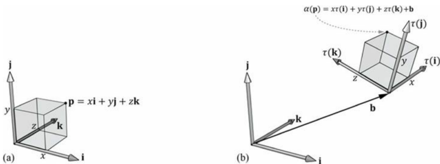
Figure 3.7. The geometry of the rows of an affine transformation matrix. The transformed point, \alpha(p) , is given as a linear combination of the transformed basis vectors \tau(\mathbf{i}) , \tau(\mathbf{j}) , \tau(\mathbf{k}) , and the offset \mathbf{b} .
