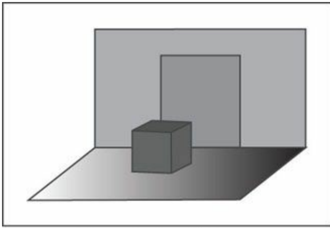
Back buffer
