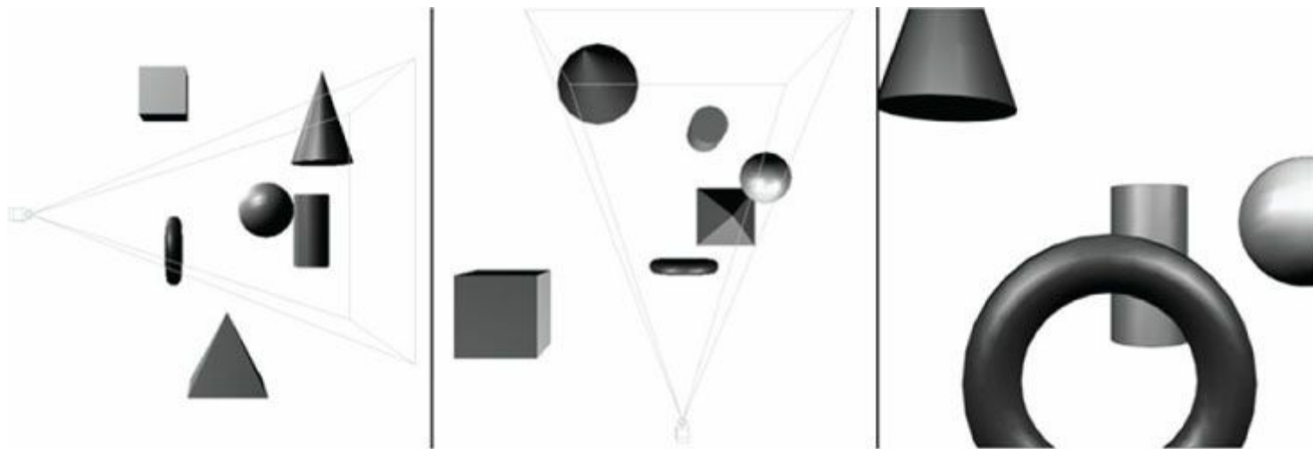
Figure 5.1. The left image shows a side view of some objects set up in the 3D world with a camera positioned and aimed; the middle image shows the same scene, but from a top-down view. The “pyramid” volume specifies the volume of space that the viewer can see; objects (and parts of objects) outside this volume are not seen. The image on the right shows the 2D image created based on what the camera “sees.”
