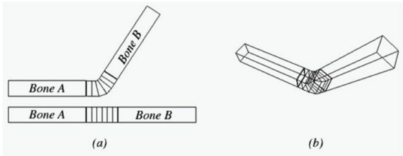
Figure 25.8. The skin is one continuous mesh that covers both bones. Observe that the vertices near the joint are influenced by both bone A and bone B to create a smooth transitional blend to simulate a flexible skin.
