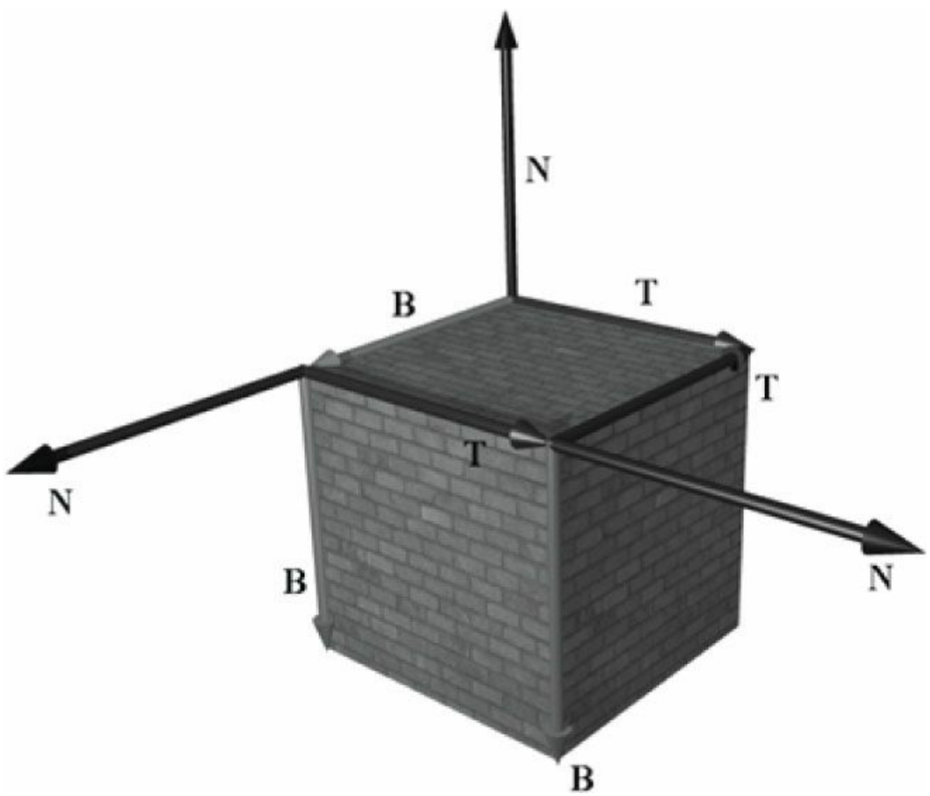
Figure 18.5. The texture space is different for each face of the box.
