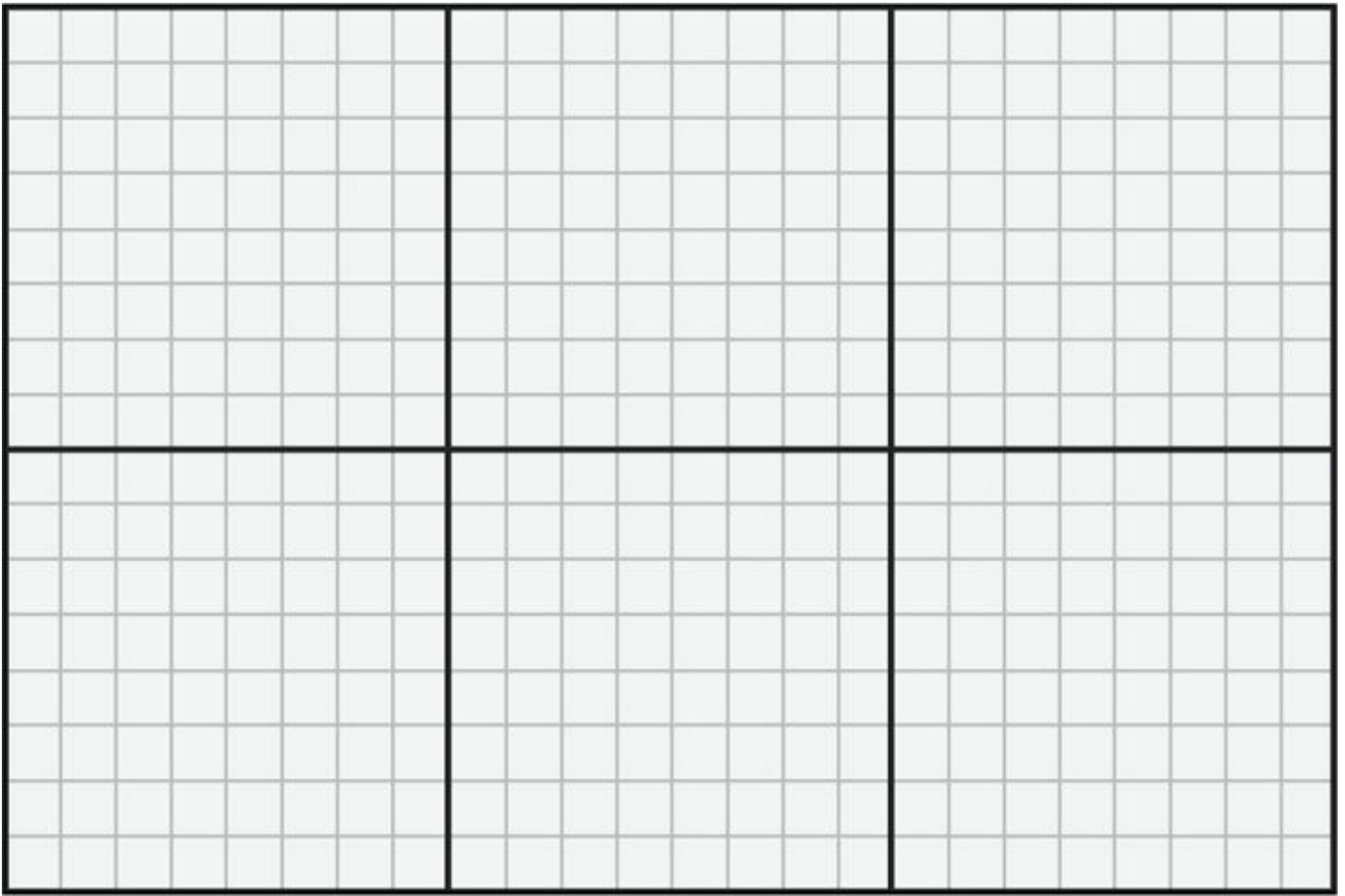
Figure 19.8. For illustration purposes, we use smaller numbers. The maximum tessellated terrain grid has 17 \times 25 vertices and 16 \times 24 cells. We divide the grid into a grid of patches such that each patch covers 8 \times 8 cells or 9 \times 9 vertices. This induces a 2 \times 3 grid of patches.
