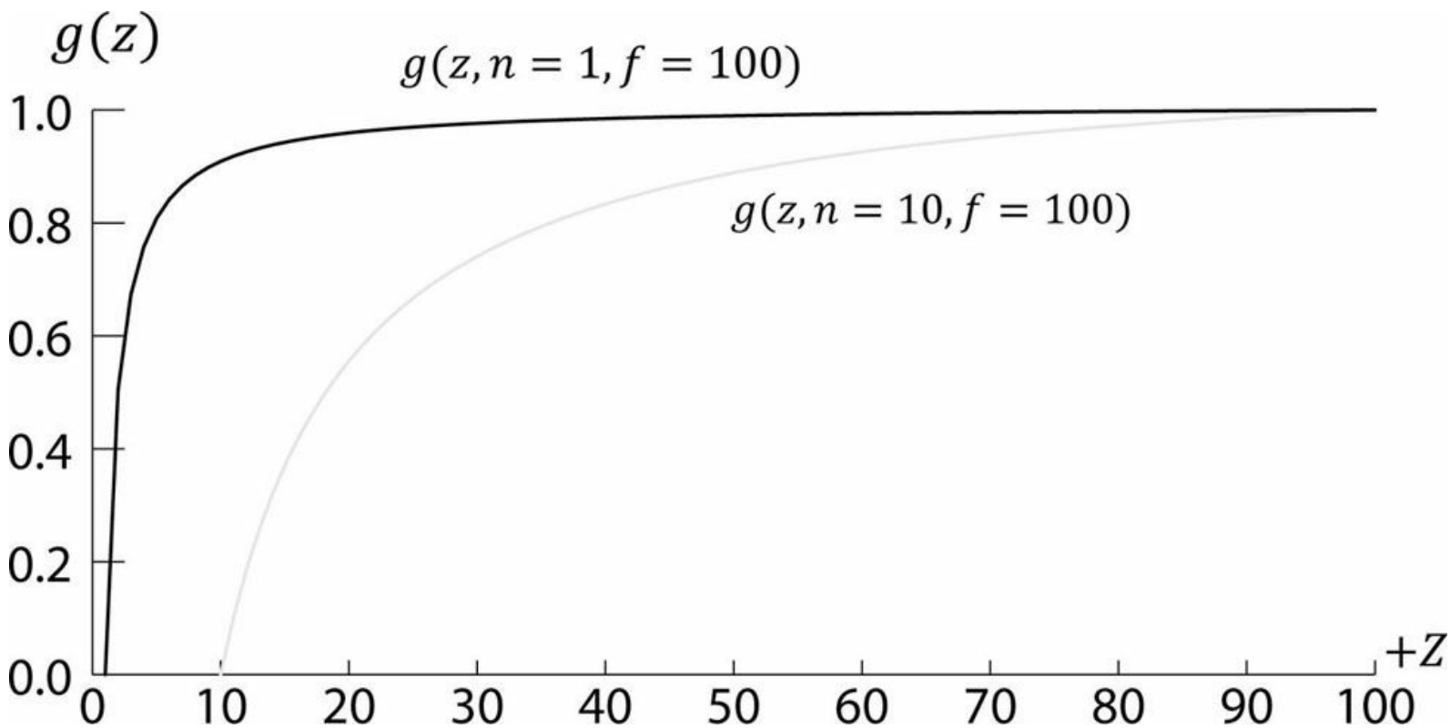
Figure 5.25. Graph of g(z) for different near planes.
