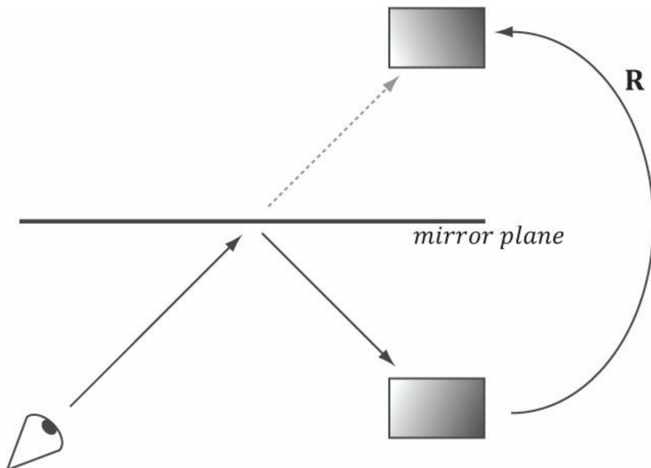
Figure 10.2. The eye sees the box reflection through the mirror. To simulate this, we reflect the box across the mirror plane and render the reflected box as usual.
