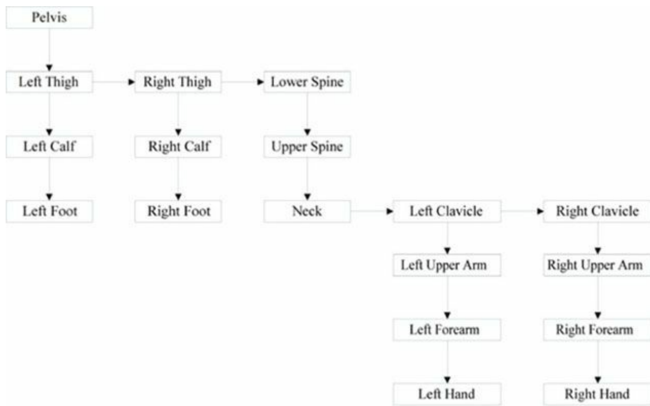
Figure 25.2. A more complex tree hierarchy to model a bipedal humanoid character. Down arrows represent “first child” relationships, and right arrows represent “sibling” relationships. For example, “Left Thigh,” “Right Thigh,” and “Lower Spine” are all children of the “Pelvis” bone.
