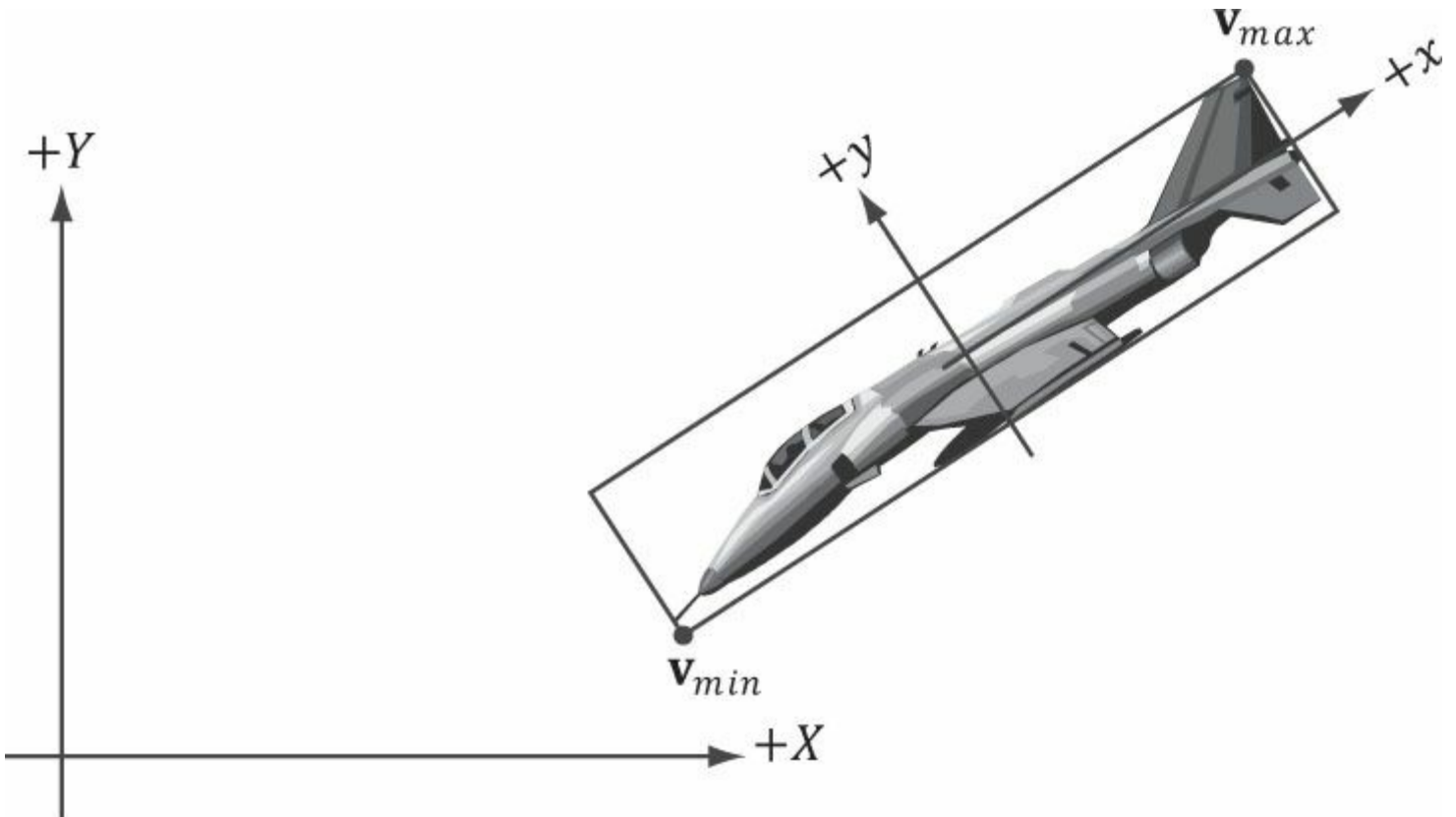
Figure 15.4. The bounding box is axis aligned with the xy -frame, but not with the XY -frame.
