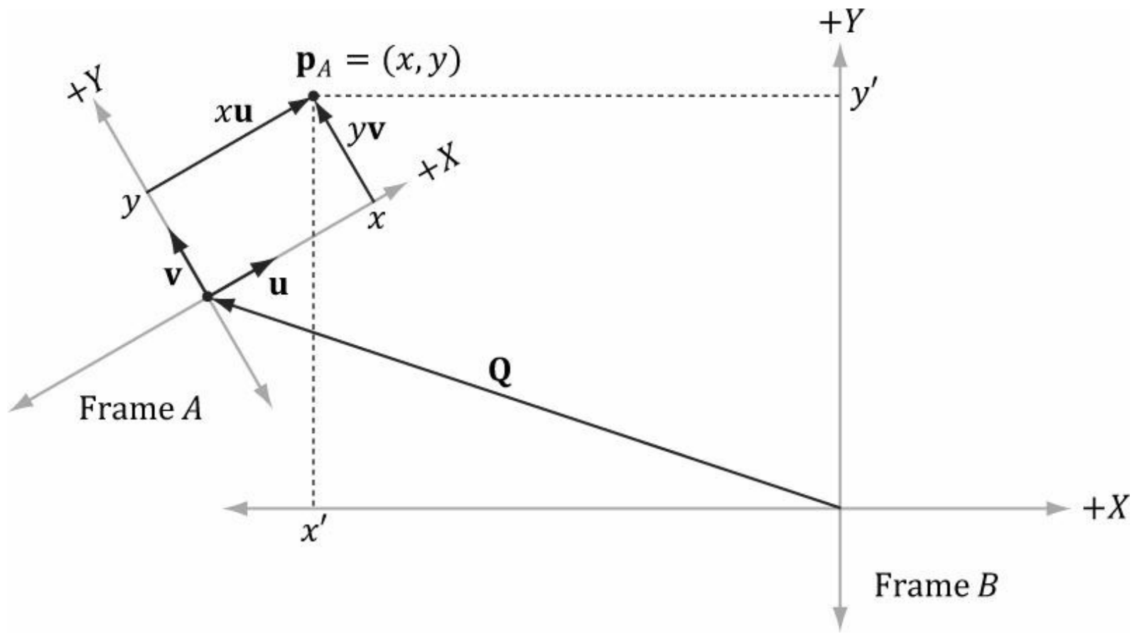
Figure 3.12. The geometry of finding the coordinates of p relative to frame B .
