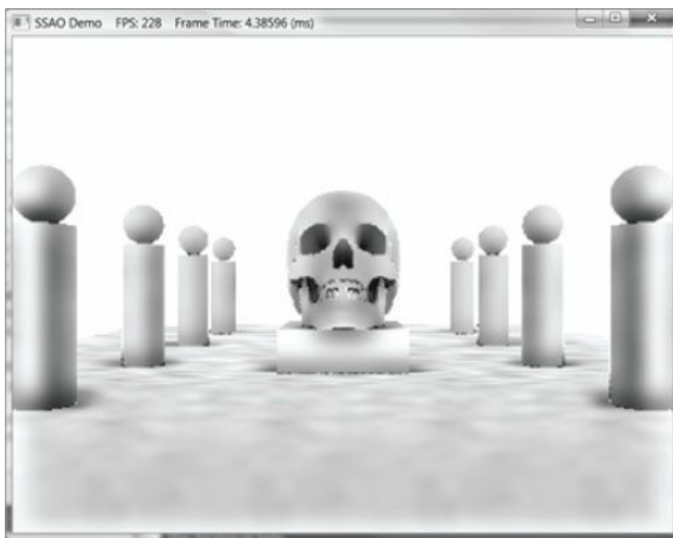
Figure 22.10. False occlusions everywhere.
