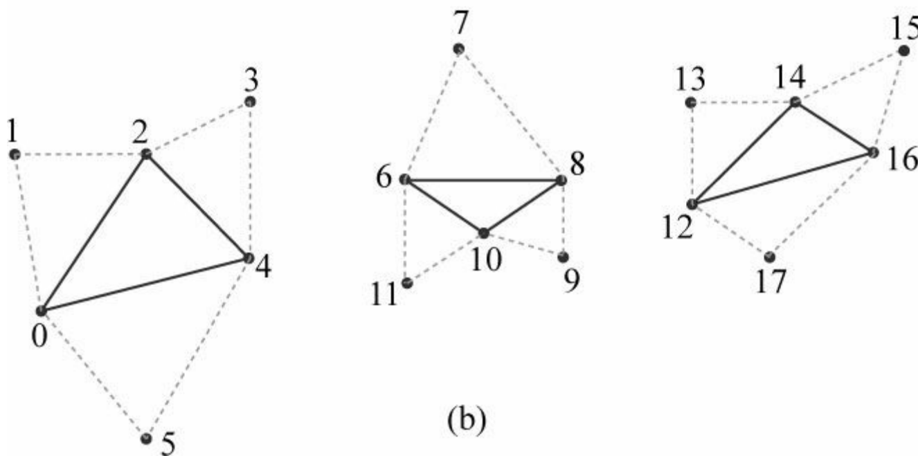
Figure 5.14. (a) A triangle list. (b) A triangle list with adjacency—observe that each triangle requires 6 vertices to describe it and its adjacent triangles. Thus 6n vertices induces n triangles with adjacency info.
