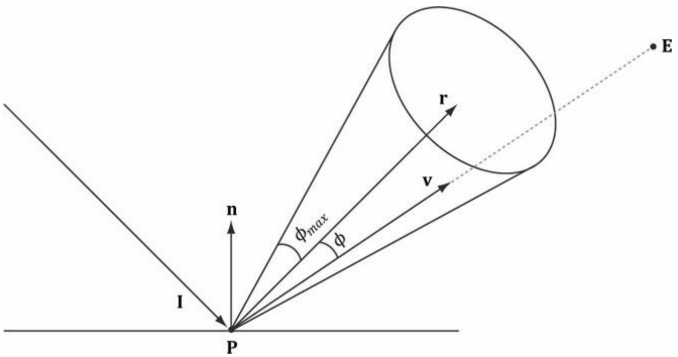
Figure 7.11. The incoming light ray is denoted by \mathbf{I} . The specular reflection does not scatter in all directions, but instead reflects in a general cone of reflection whose size we can control with a parameter. If \mathbf{v} is in the cone, the eye receives specular light; otherwise, it does not. The closer is aligned with the reflection vector \mathbf{r} , the more specular light the eye receives.
