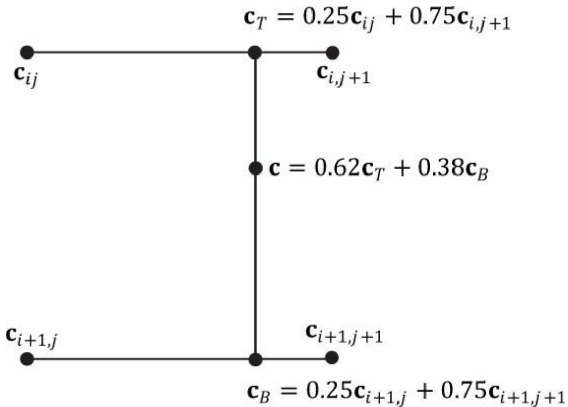
Figure 8.6. Here we have four texel points c_{ij} , c_{i,j+1} , c_{i+1,j} , and c_{i+1,j+1} . We want to approximate the color of c , which lies between these four texel points using interpolation; in this example, c lies 0.75 units to the right of c_{ij} and 0.38 units below c_{ij} . We first do a 1D linear interpolation between the top two colors to get c_T . Likewise, we do a 1D linear interpolate between the bottom two colors to get c_B . Finally, we do a 1D linear interpolation between c_T and c_B to get c .
