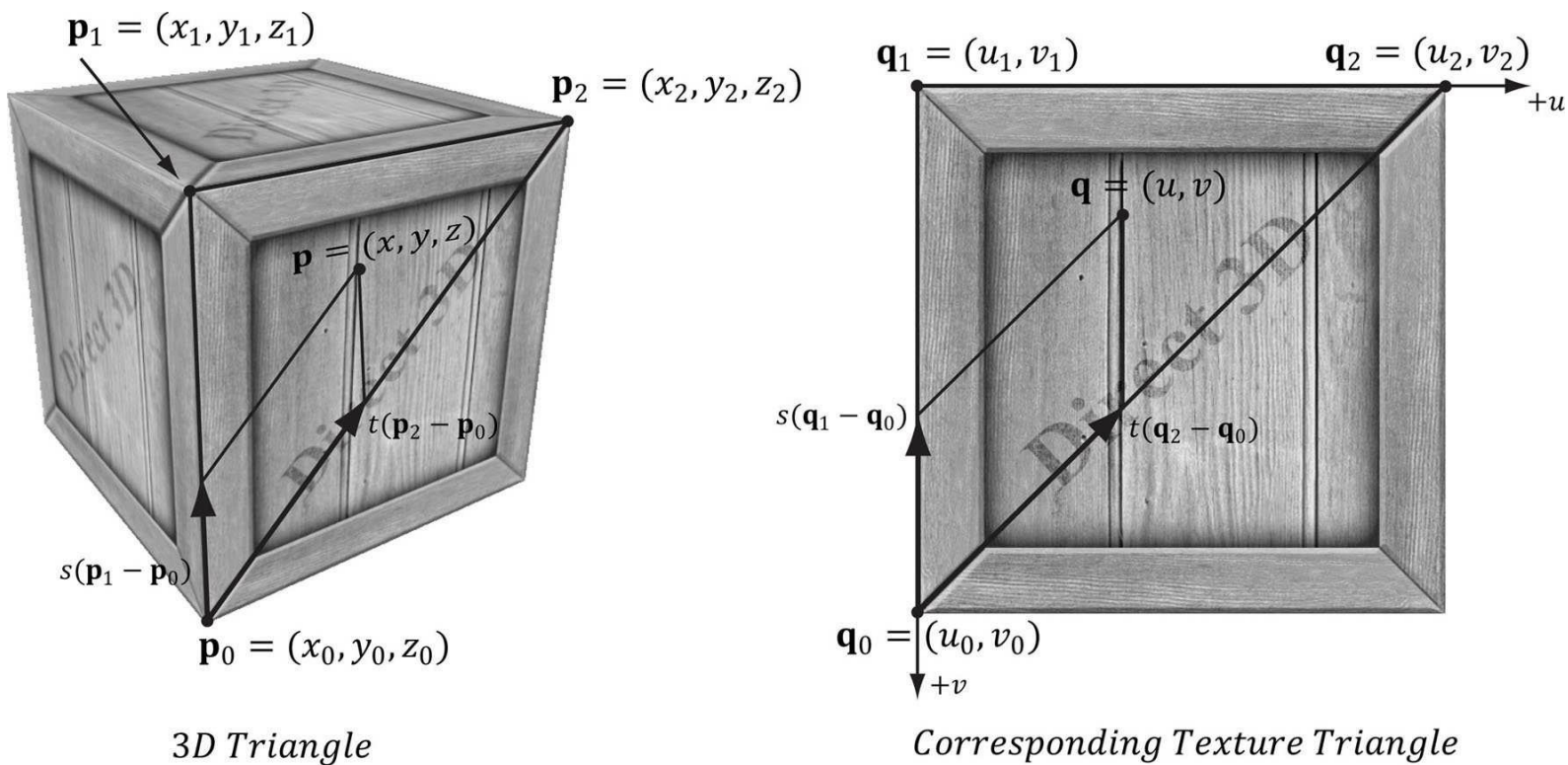
Figure 8.3. On the left is a triangle in 3D space, and on the right we define a 2D triangle on the texture that is going to be mapped onto the 3D triangle.
