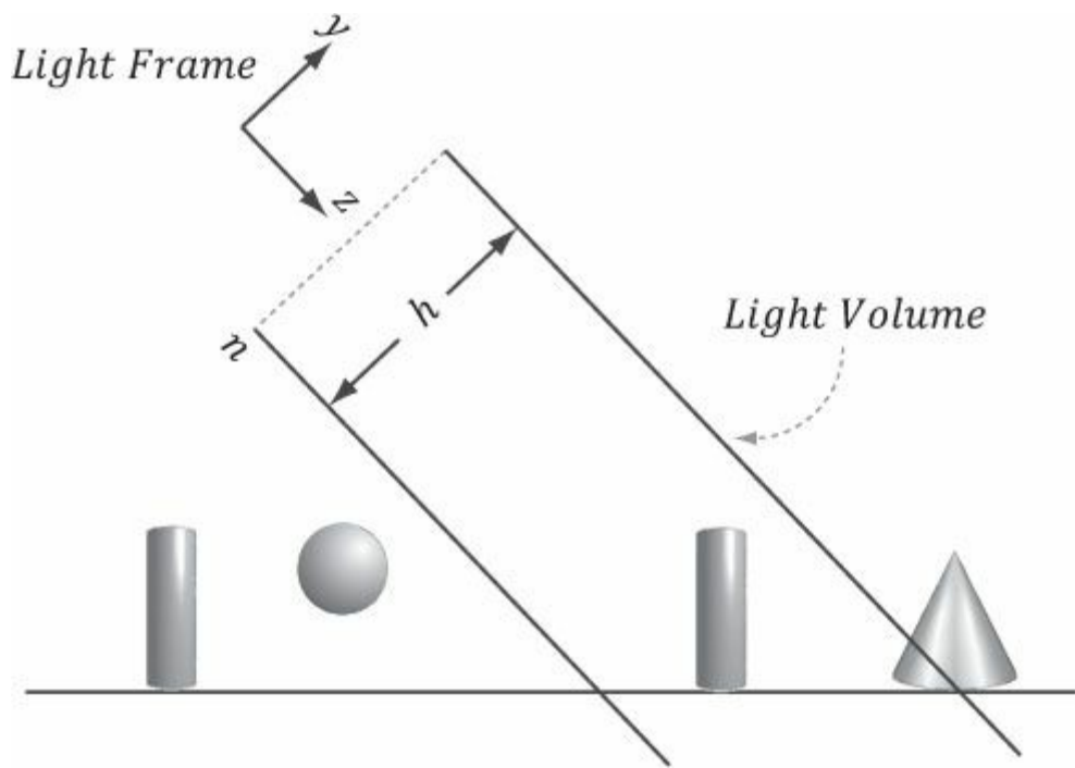
Figure 21.5. Parallel light rays travel through the light volume, so only a subset of the scene inside the volume receives light. If the light source needs to strike the entire scene, we can set the light volume size to contain the entire scene.
