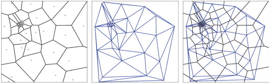
Figure 6.3. A 2D Voronoi diagram of a point set (left), 2D Delaunay triangulation of the same point set (center), and both superimposed (right).
